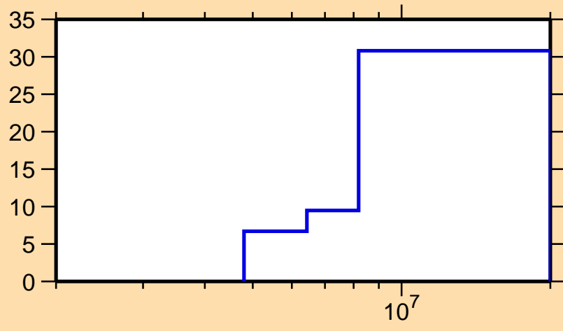
\Delta\sigma/\sigma vs. E for ^{30}\text{Al}(n,inel.)
