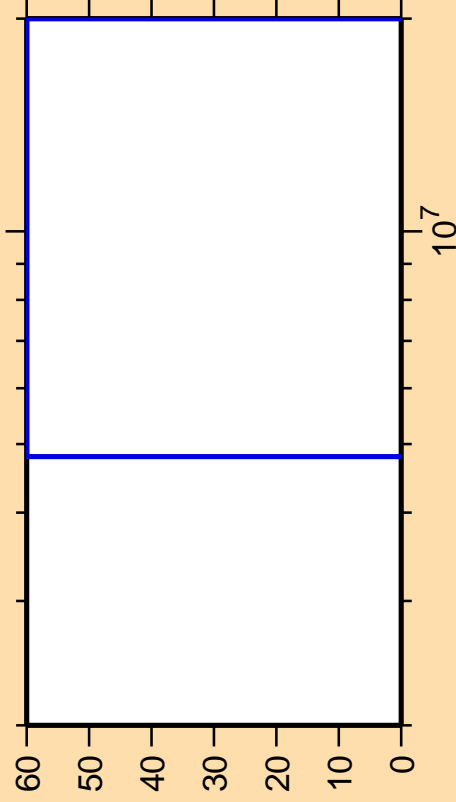
\Delta\sigma/\sigma vs. E for ^{30}\text{Al}(n,ncont.)
