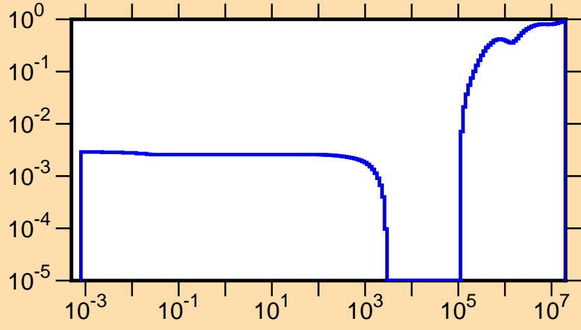
\mu vs. E for ^{231}\text{Am}(\text{mt251})
