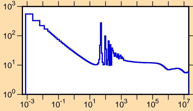
\sigma vs. E for ^{231}\text{Am}(n,\text{tot.})
