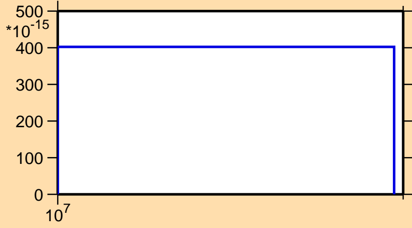
\sigma vs. E for ^{231}\text{Am}(n,2np)
