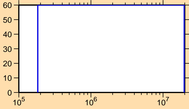
\Delta\sigma/\sigma vs. E for ^{231}\text{Am}(n,n_1)
