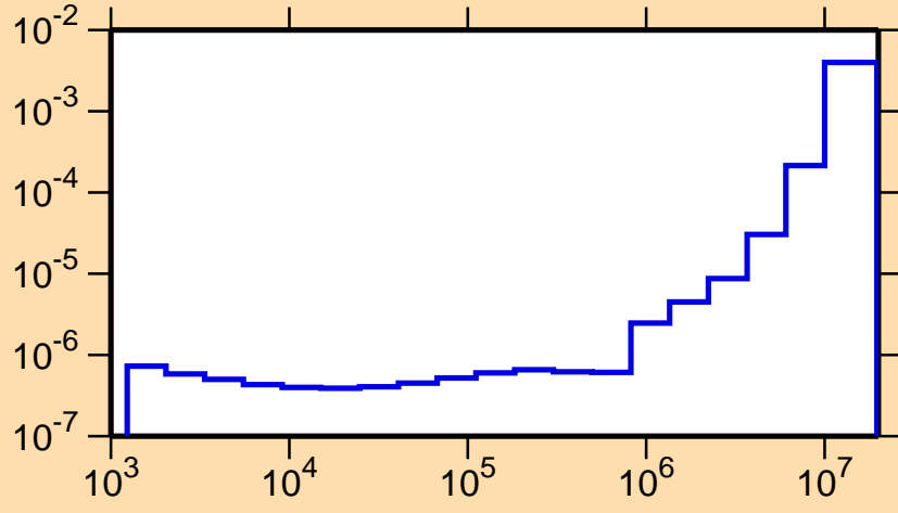
\sigma vs. E for ^{231}\text{Am}(n,\alpha)
