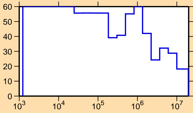
\Delta\sigma/\sigma vs. E for ^{231}\text{Am}(n,el.)
