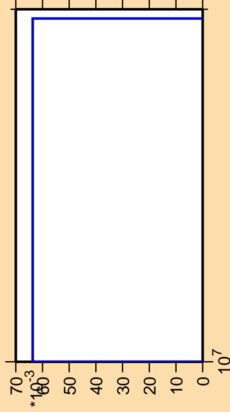
\Delta\sigma/\sigma vs. E for ^{231}\text{Am} (mt 34)
