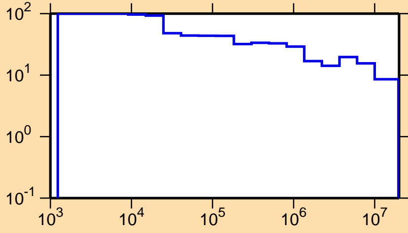
\Delta\sigma/\sigma vs. E for ^{231}\text{Am}(n,\text{tot.})
