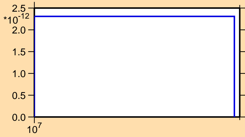
\sigma vs. E for ^{231}\text{Am}(n,\text{nd})
