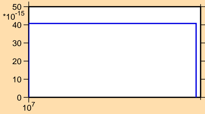
\sigma vs. E for ^{231}\text{Am} (mt 34)
