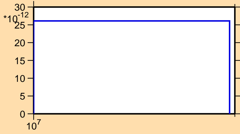
\sigma vs. E for ^{231}\text{Am}(n,3n)
