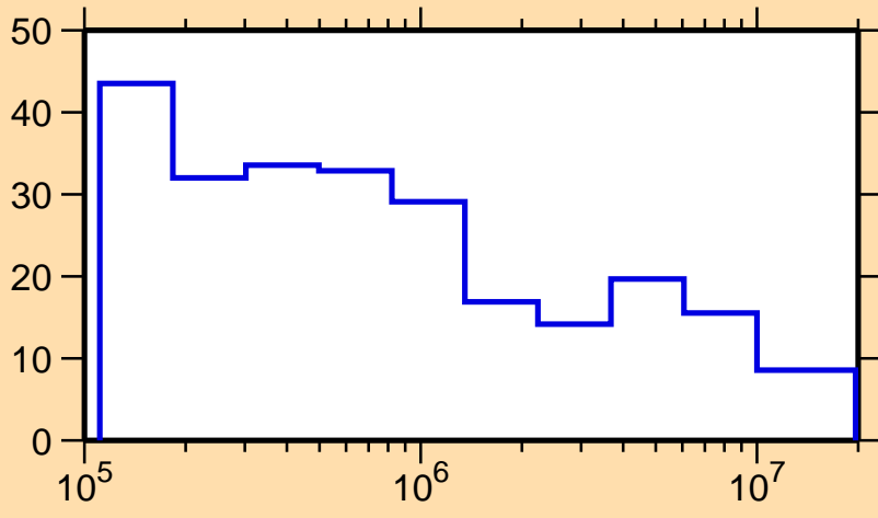
\Delta\sigma/\sigma vs. E for ^{231}\text{Am}(n,\text{tot.})
