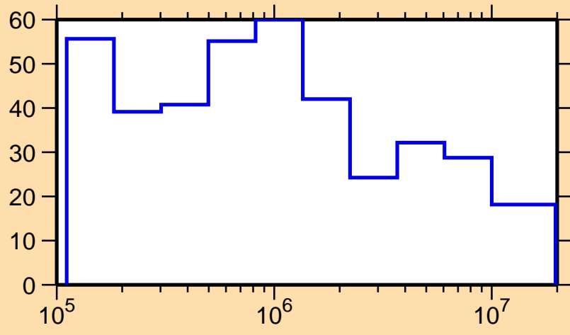
\Delta\sigma/\sigma vs. E for ^{231}\text{Am}(n,\text{el.})
