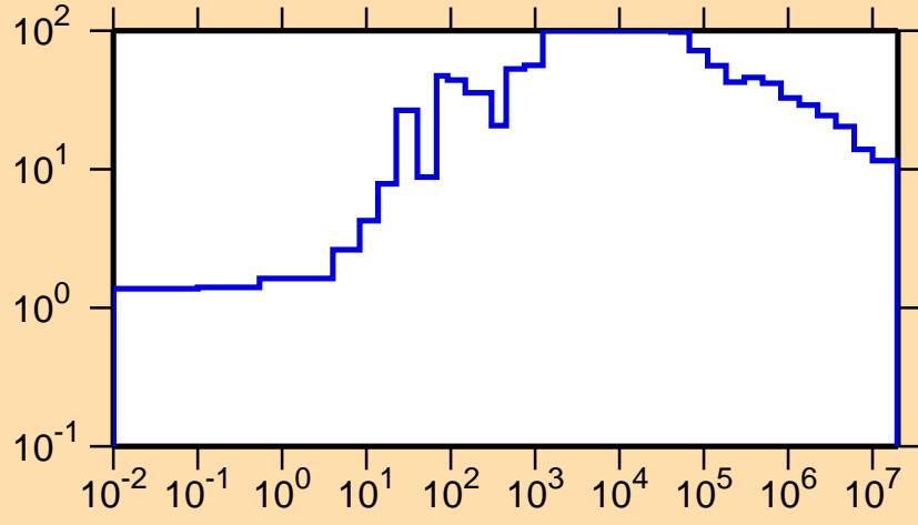
\Delta\sigma/\sigma vs. E for ^{231}\text{Am}(n,f)
