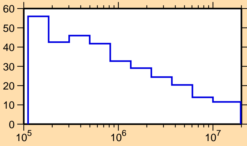
\Delta\sigma/\sigma vs. E for ^{231}\text{Am}(n,f)
