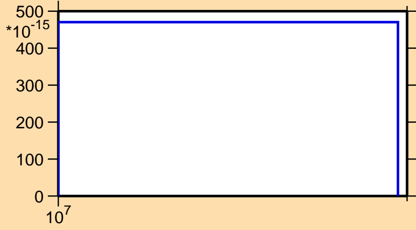
\sigma vs. E for ^{231}\text{Am}(n,nt)
