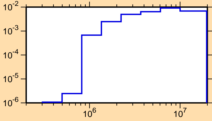
\sigma vs. E for ^{231}\text{Am}(n,n\alpha)
