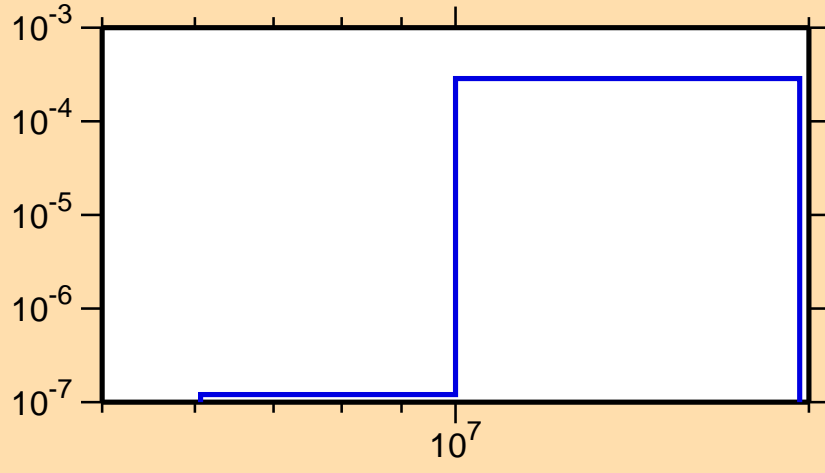
\sigma vs. E for ^{231}\text{Am}(n,2n\alpha)
