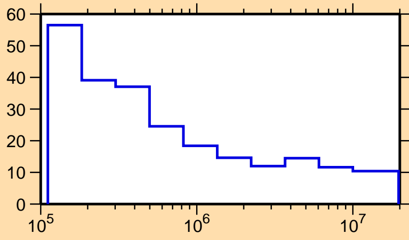
\Delta\sigma/\sigma vs. E for ^{231}\text{Am}(n,\text{nonel.})
