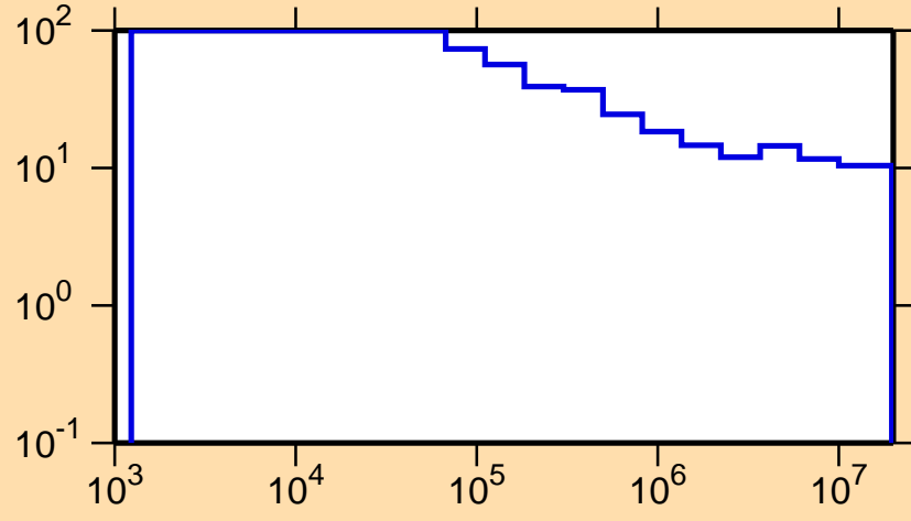
\Delta\sigma/\sigma vs. E for ^{231}\text{Am}(n,\text{nonel.})
