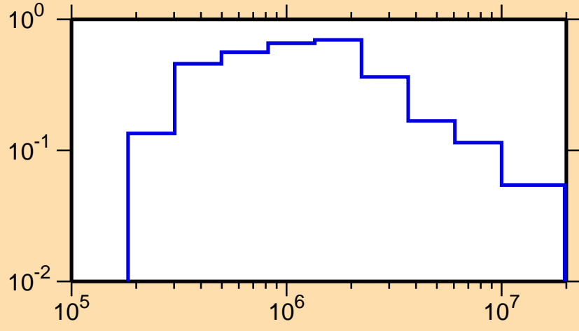
\sigma vs. E for ^{231}\text{Am}(n,\text{inel.})
