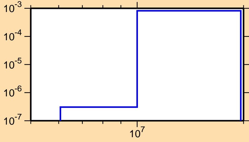
\sigma vs. E for ^{231}\text{Am}(n,2n)
