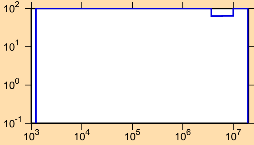
\Delta\sigma/\sigma vs. E for ^{231}\text{Am}(n,p)
