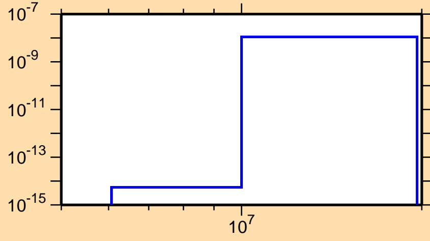
\sigma vs. E for ^{231}\text{Am}(n,\text{He3})
