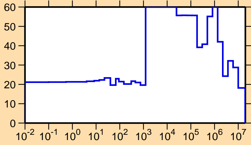
\Delta\sigma/\sigma vs. E for ^{231}\text{Am}(n,el.)
