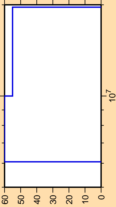
\Delta\sigma/\sigma vs. E for ^{231}\text{Am}(n,\alpha)
