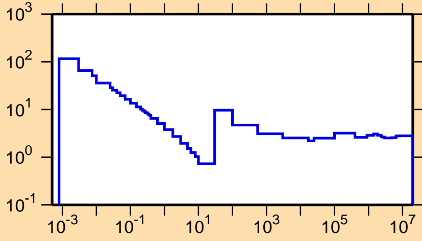
\sigma vs. E for ^{231}\text{Am}(n,f)
