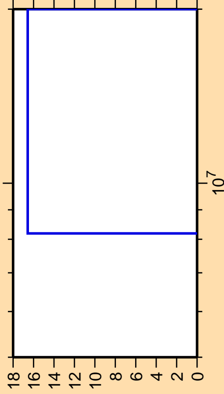
\Delta\sigma/\sigma vs. E for ^{231}\text{Am}(n,nd)
