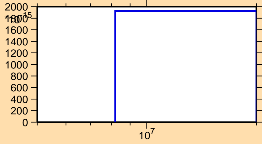
\sigma vs. E for ^{231}\text{Am}(n,nd)
