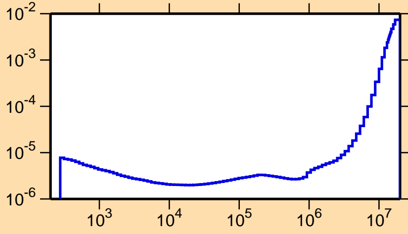
\sigma vs. E for ^{233}\text{Am}(n,\alpha)
