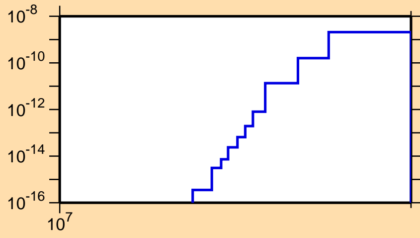
\sigma vs. E for ^{233}\text{Am}(n,2np)
