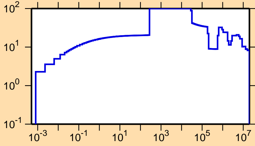
\Delta\sigma/\sigma vs. E for ^{233}\text{Am}(n,tot.)
