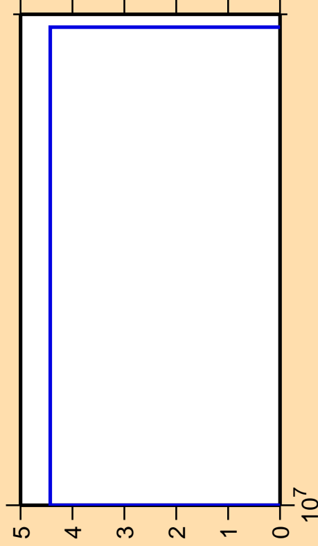
\Delta\sigma/\sigma vs. E for ^{233}\text{Am}(n,nt)
