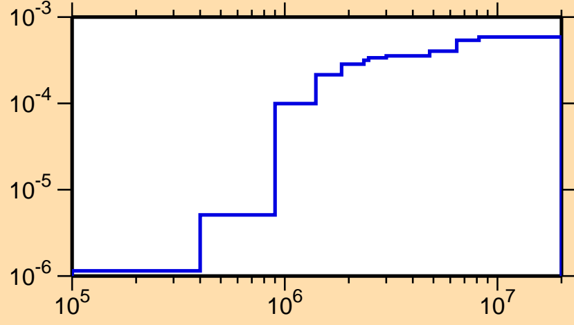
\sigma vs. E for ^{233}\text{Am}(n,n\alpha)
