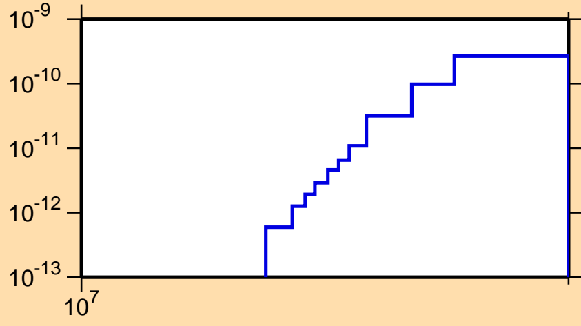
\sigma vs. E for ^{235}\text{Am}(\text{mt117})
