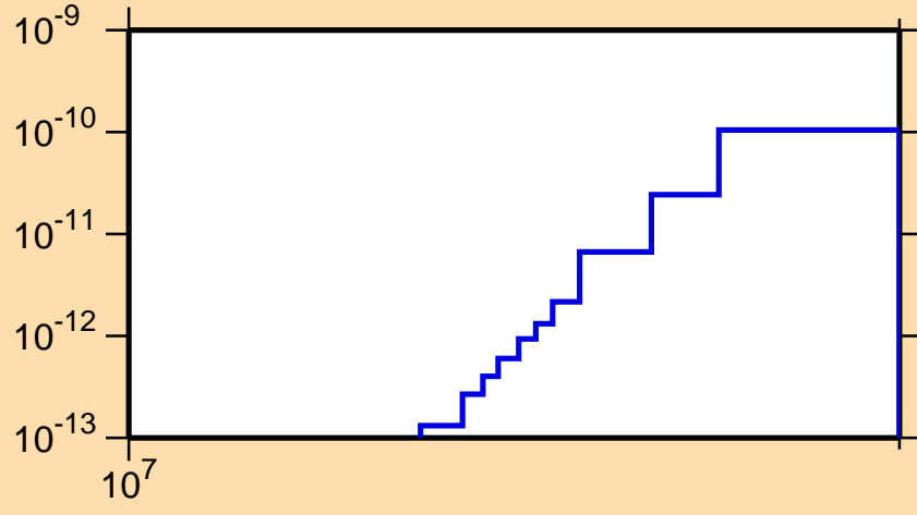
\sigma vs. E for ^{235}\text{Am} (mt 45)
