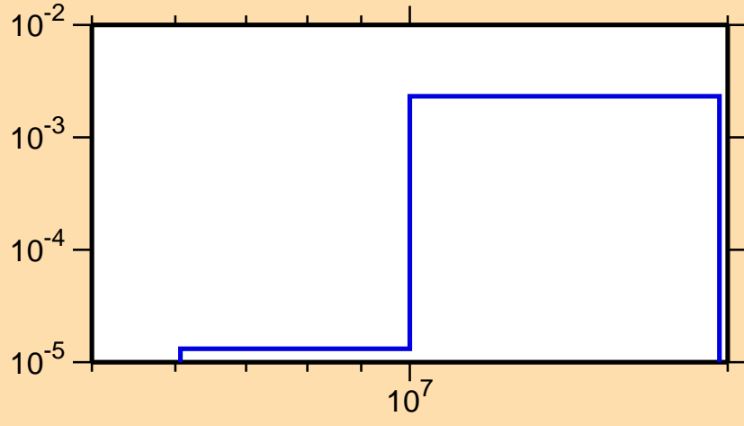
\sigma vs. E for ^{235}\text{Am}(n,2n\alpha)
