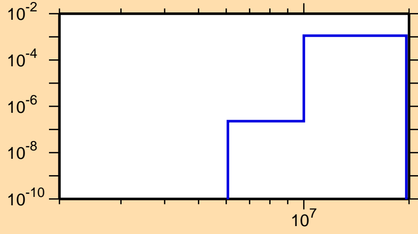
\sigma vs. E for ^{235}\text{Am}(n,d)
