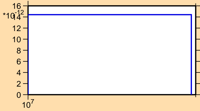
\sigma vs. E for ^{235}\text{Am}(\text{mt117})
