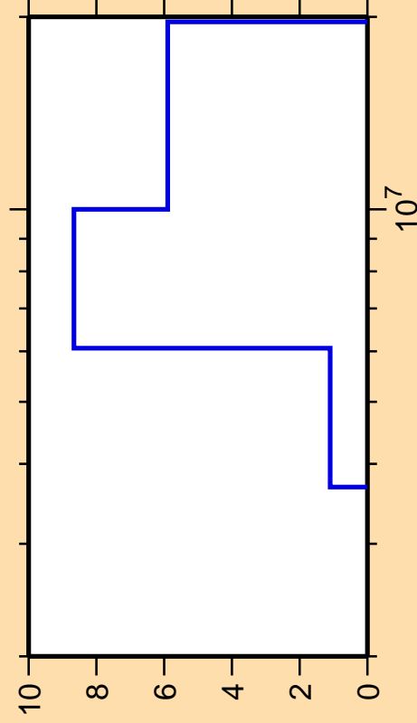
\Delta\sigma/\sigma vs. E for ^{235}\text{Am}(n,d)
