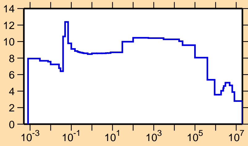
\sigma vs. E for ^{235}\text{Am}(n,\text{el.})
