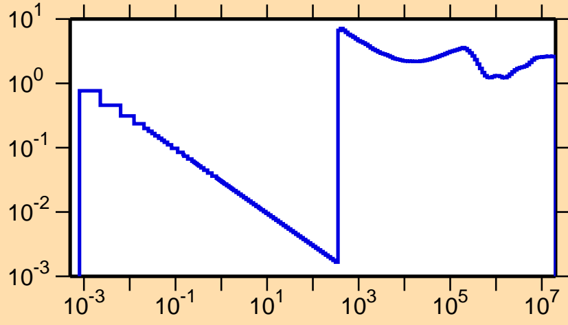
\sigma vs. E for ^{236}\text{Am}(n,f)
