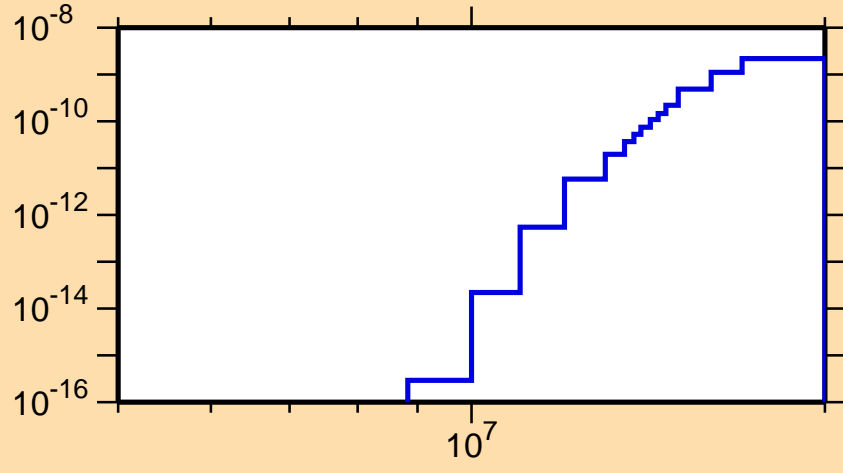
\sigma vs. E for ^{236}\text{Am}(\text{mt117})
