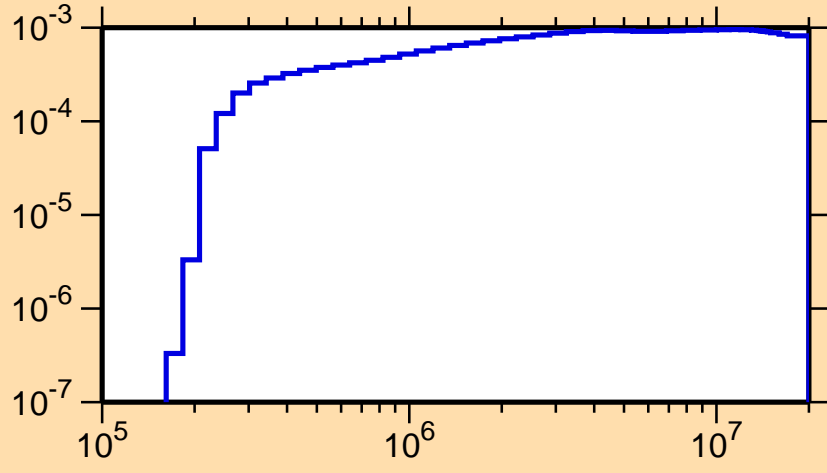
\sigma vs. E for ^{236}\text{Am}(n,n_1)
