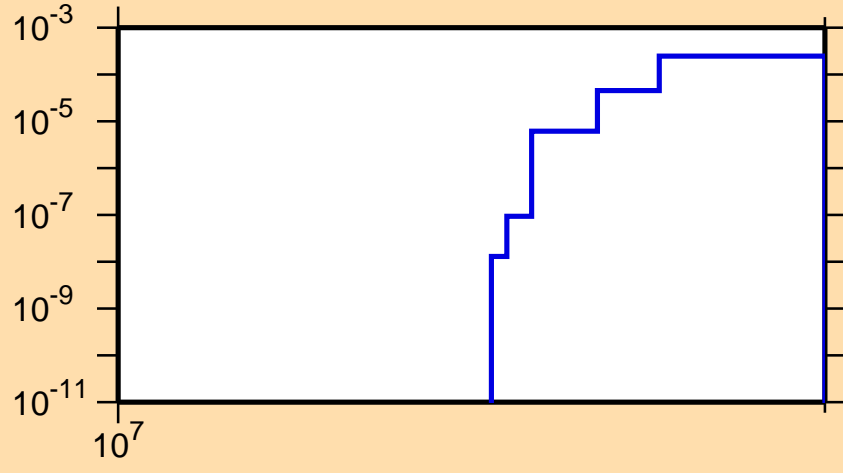
\sigma vs. E for ^{236}\text{Am}(n,3n\alpha)
