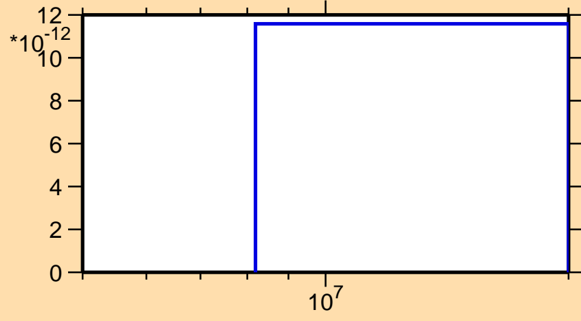
\sigma vs. E for ^{236}\text{Am} (mt 45)
