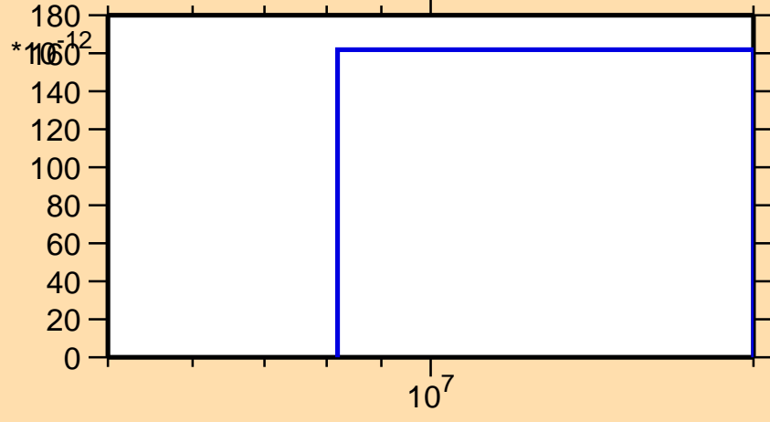
\sigma vs. E for ^{236}\text{Am}(\text{mt117})
