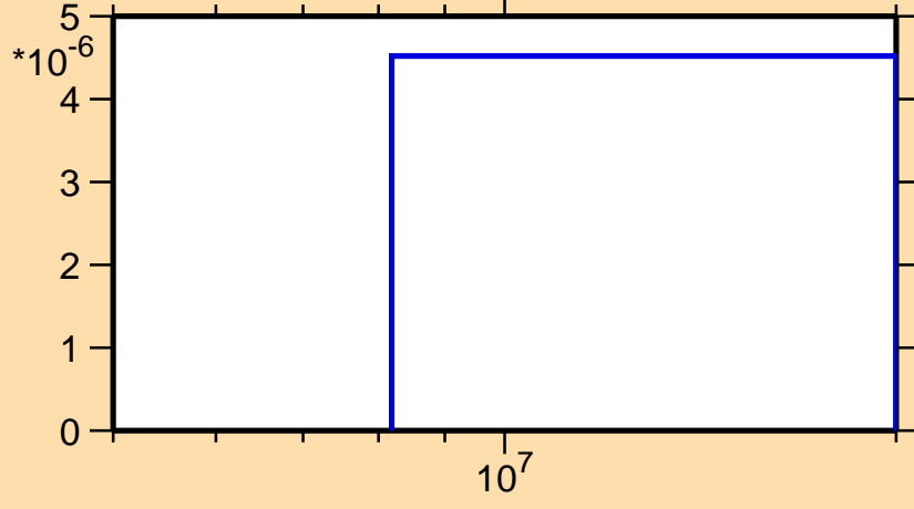
\sigma vs. E for ^{236}\text{Am}(n,3n\alpha)
