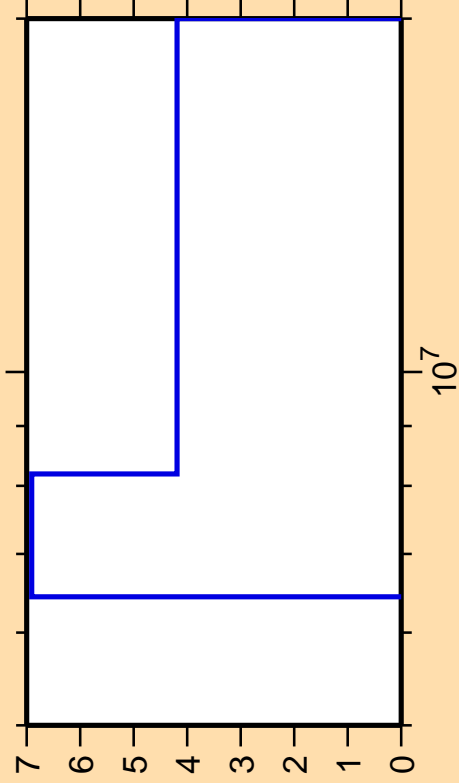
\Delta\sigma/\sigma vs. E for ^{236}\text{Am}(n,n\text{cont.})
