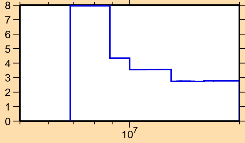
\Delta\sigma/\sigma vs. E for ^{237}\text{Am}(n,\text{tot.})
