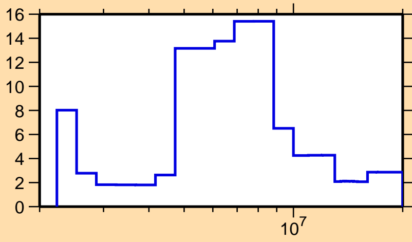
\Delta\sigma/\sigma vs. E for ^{237}\text{Am}(n, el.)
