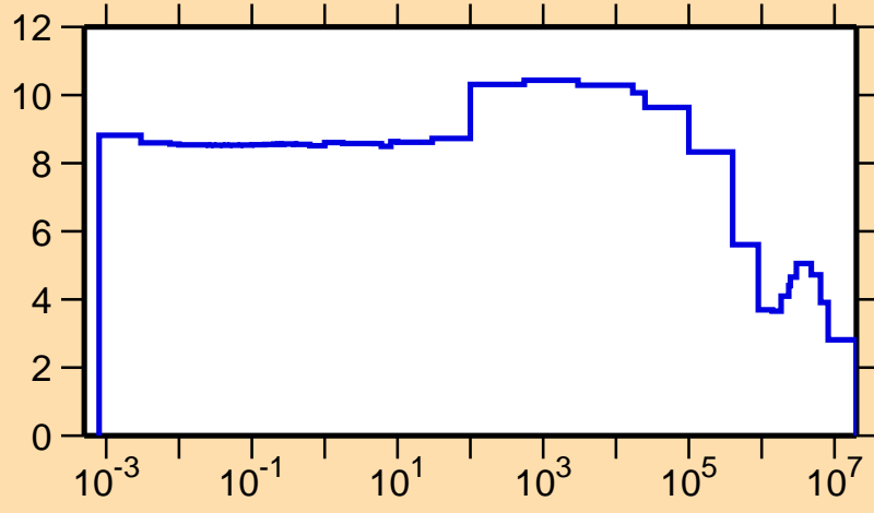
\sigma vs. E for ^{237}\text{Am}(n,\text{el.})
