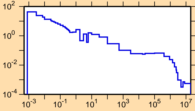
\sigma vs. E for ^{237}\text{Am}(n,\gamma)
