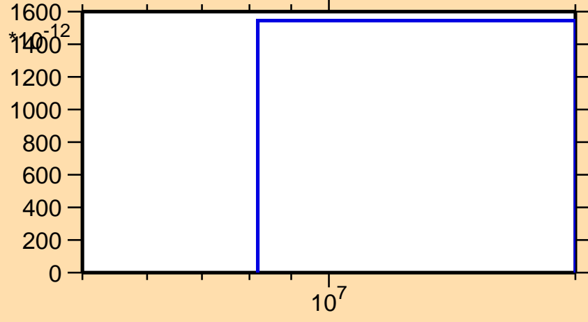
\sigma vs. E for ^{237}\text{Am}(\text{mt117})
