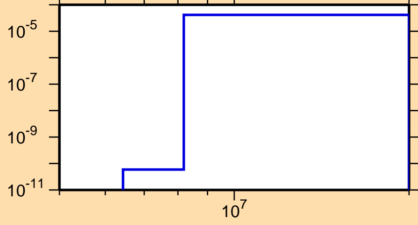
\sigma vs. E for ^{237}\text{Am}(n,np)
