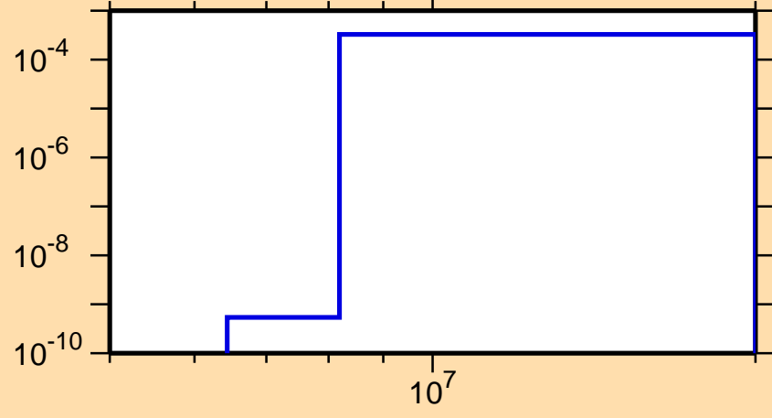
\sigma vs. E for ^{237}\text{Am}(n,d)
