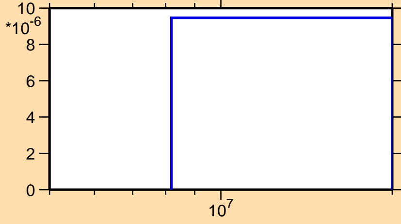
\sigma vs. E for ^{237}\text{Am}(n,3n\alpha)
