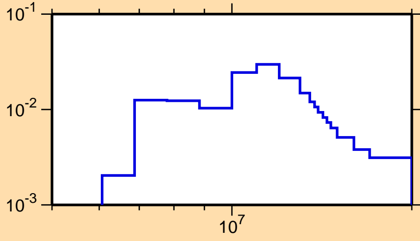
\sigma vs. E for ^{238}\text{Am}(n,2n)
