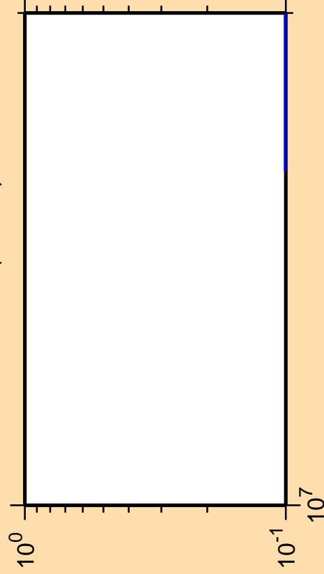
\Delta\sigma/\sigma vs. E for ^{238}\text{Am} (mt 34)
