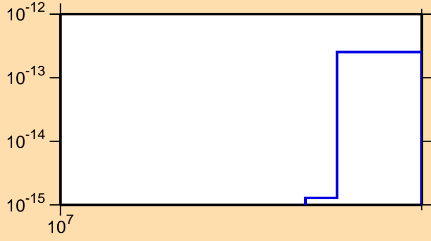
\sigma vs. E for ^{238}\text{Am} (mt 34)
