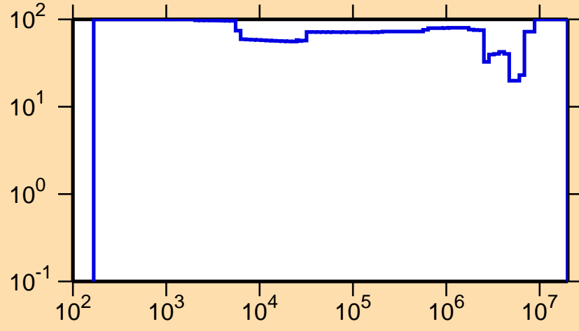
\Delta\sigma/\sigma vs. E for ^{238}\text{Am}(n,\gamma)
