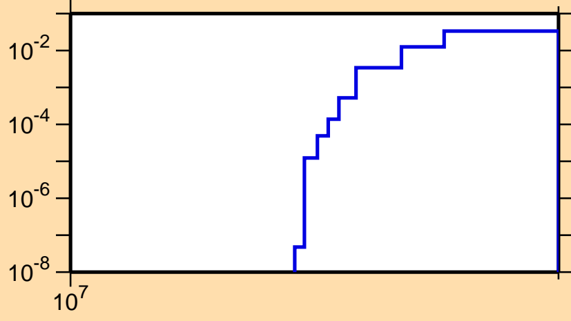
\sigma vs. E for ^{238}\text{Am}(n,3n)
