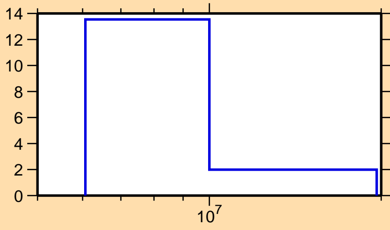
\Delta\sigma/\sigma vs. E for ^{238}\text{Am}(n,\text{tot.})
