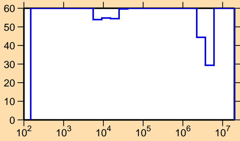
\Delta\sigma/\sigma vs. E for ^{238}\text{Am}(n,\gamma)
