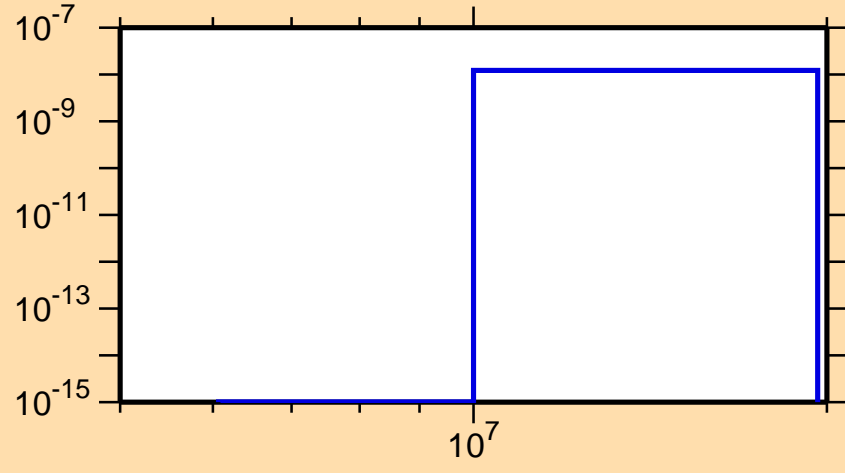
\sigma vs. E for ^{238}\text{Am}(\text{mt117})
