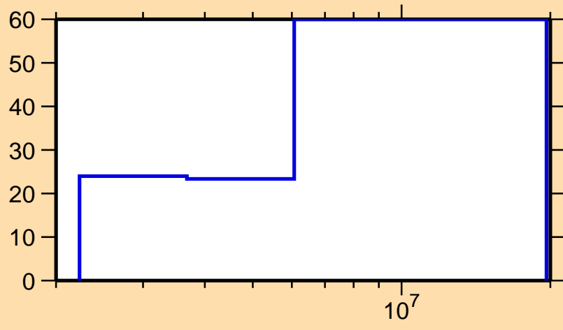
\Delta\sigma/\sigma vs. E for ^{238}\text{Am}(n,n_1)
