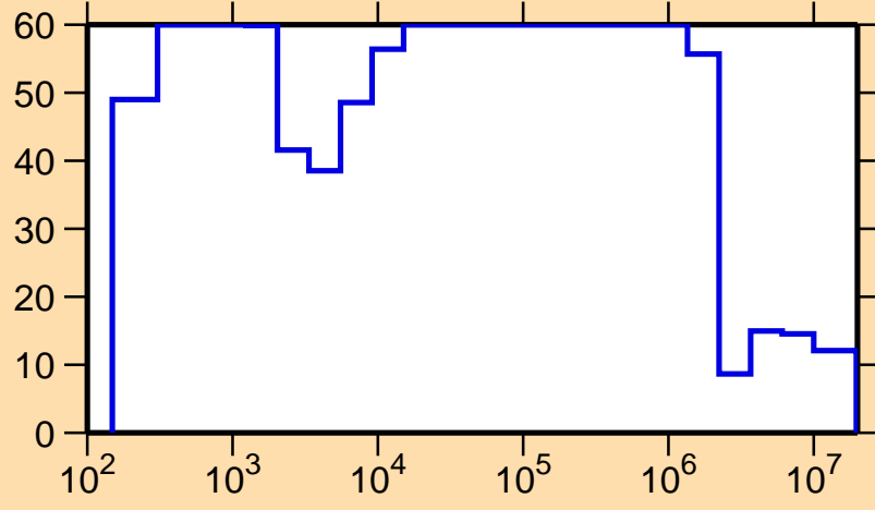
\Delta\sigma/\sigma vs. E for ^{238}\text{Am}(n,p)
