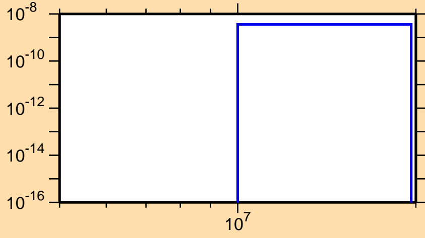
\sigma vs. E for ^{238}\text{Am} (mt 45)
