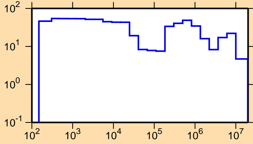
\Delta\sigma/\sigma vs. E for ^{238}\text{Am}(n,el.)
