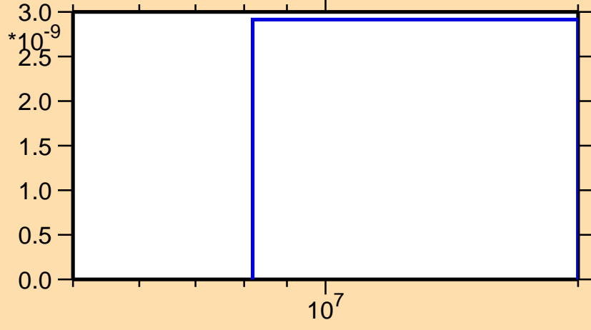
\sigma vs. E for ^{238}\text{Am} (mt 45)
