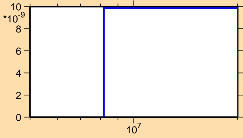
\sigma vs. E for ^{238}\text{Am}(\text{mt117})
