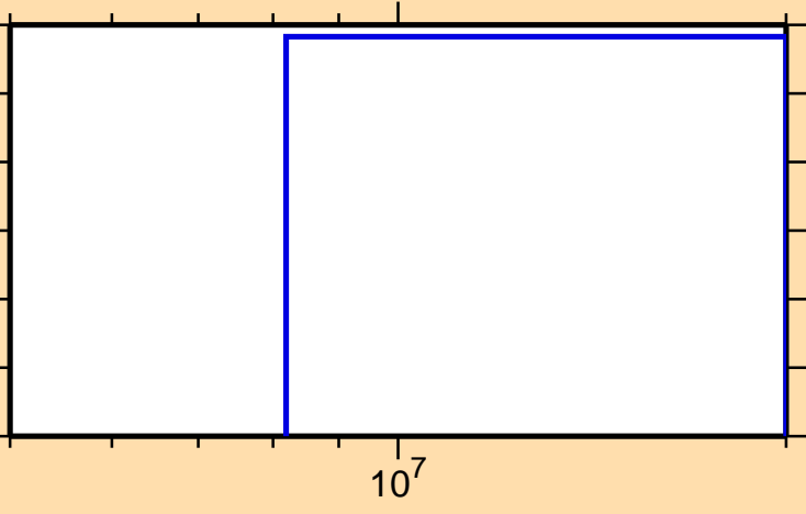
\sigma vs. E for ^{238}\text{Am} (mt 45)
