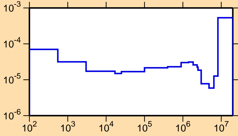
\sigma vs. E for ^{238}\text{Am}(n,\alpha)
