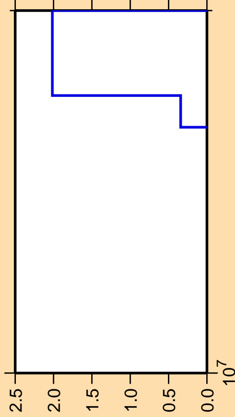
\Delta\sigma/\sigma vs. E for ^{240}\text{Am} (mt 45)
