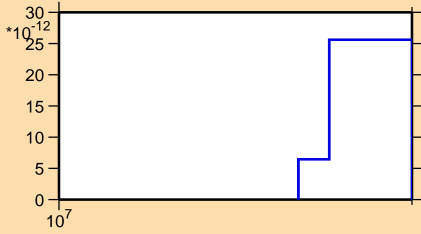
\sigma vs. E for ^{240}\text{Am}(\text{mt117})
