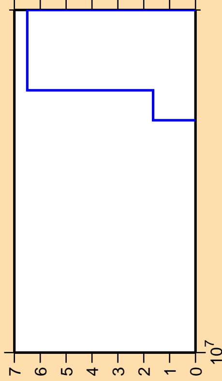
\Delta\sigma/\sigma vs. E for ^{240}\text{Am}(\text{mt117})
