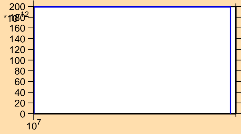
\sigma vs. E for ^{240}\text{Am}(n,p\alpha)
