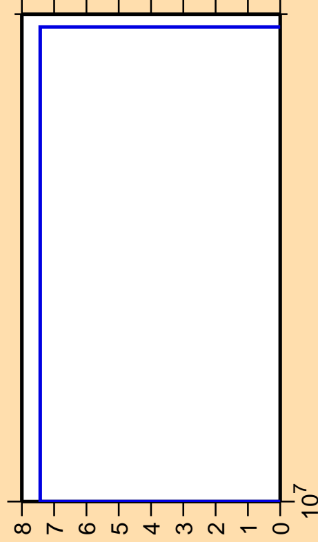
\Delta\sigma/\sigma vs. E for ^{240}\text{Am}(n,3n)
