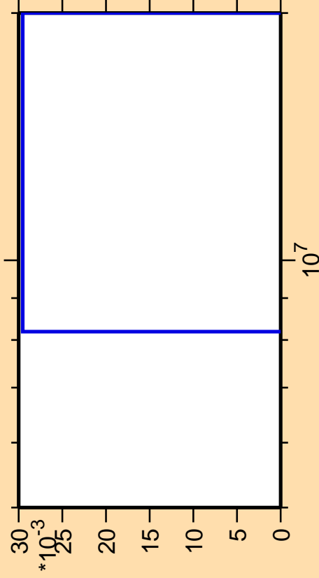
\Delta\sigma/\sigma vs. E for ^{240}\text{Am} (mt 45)
