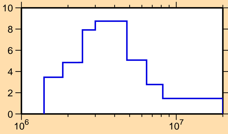
\Delta\sigma/\sigma vs. E for ^{240}\text{Am}(n,f)
