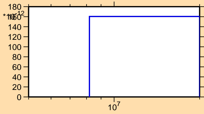
\sigma vs. E for ^{240}\text{Am}(n,p\alpha)
