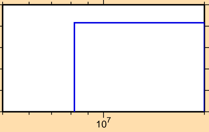
\sigma vs. E for ^{240}\text{Am}(\text{mt117})
