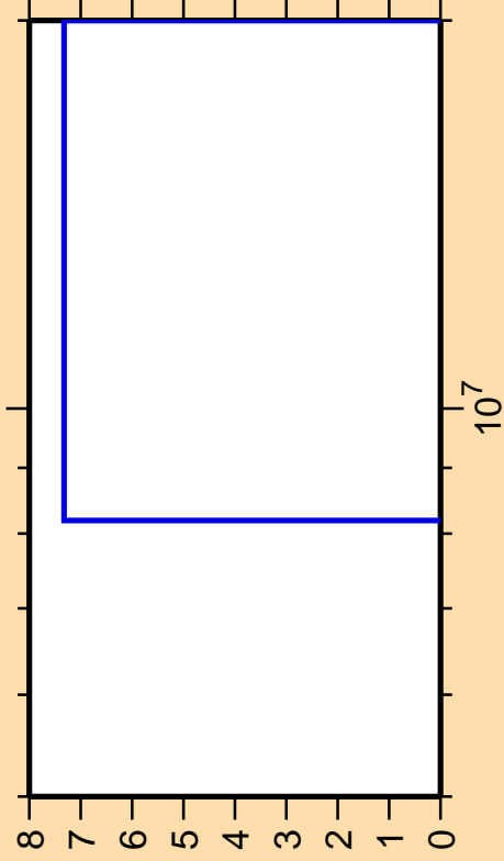
\Delta\sigma/\sigma vs. E for ^{240}\text{Am}(n,nt)
