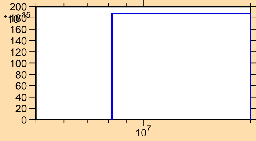
\sigma vs. E for ^{240}\text{Am} (mt 45)
