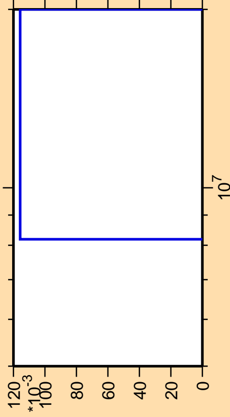
\Delta\sigma/\sigma vs. E for ^{240}\text{Am}(\text{mt117})
