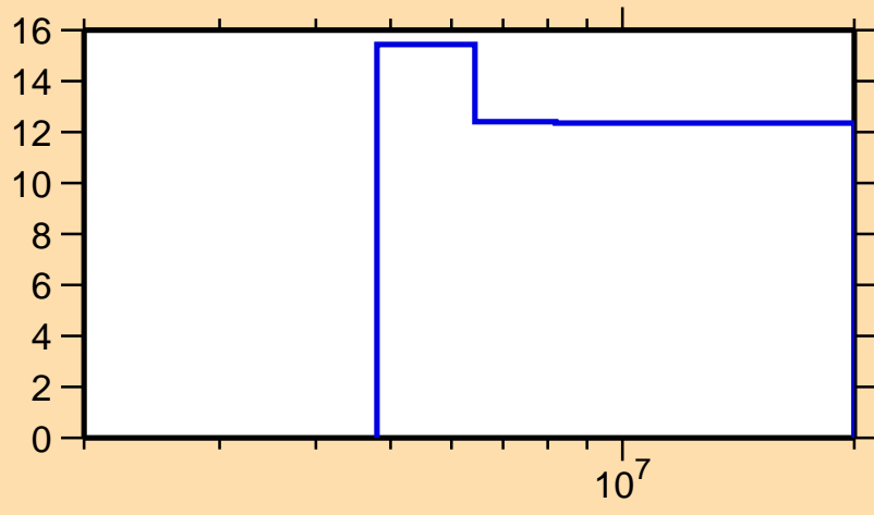
\Delta\sigma/\sigma vs. E for ^{240}\text{Am}(n,2n)
