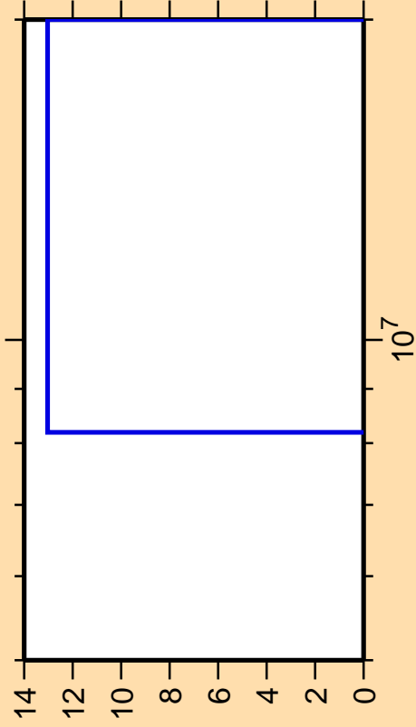
\Delta\sigma/\sigma vs. E for ^{240}\text{Am}(n,p\alpha)
