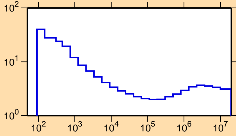
\sigma vs. E for ^{241}\text{Am}(n,\text{nonel.})
