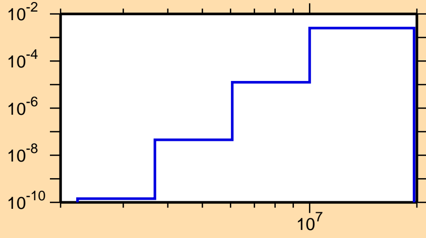
\sigma vs. E for ^{241}\text{Am}(n,p)
