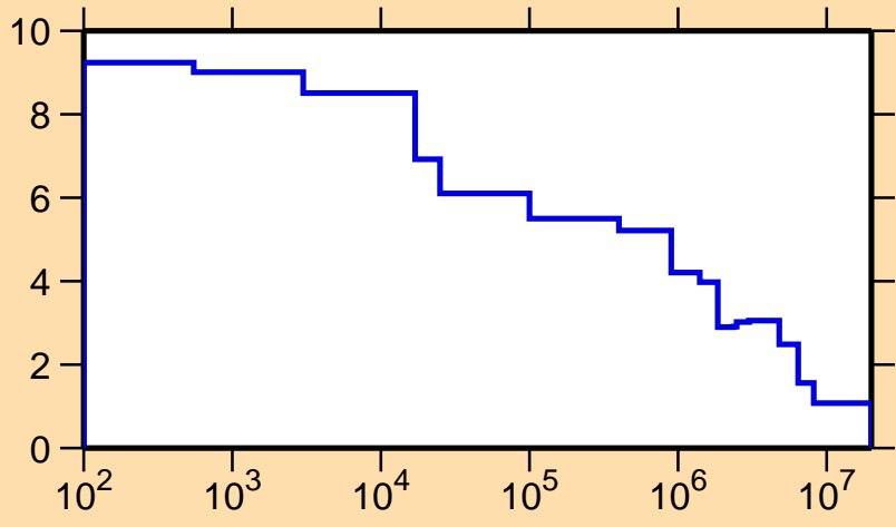
\Delta\sigma/\sigma vs. E for ^{241}\text{Am}(n,\text{nonel.})
