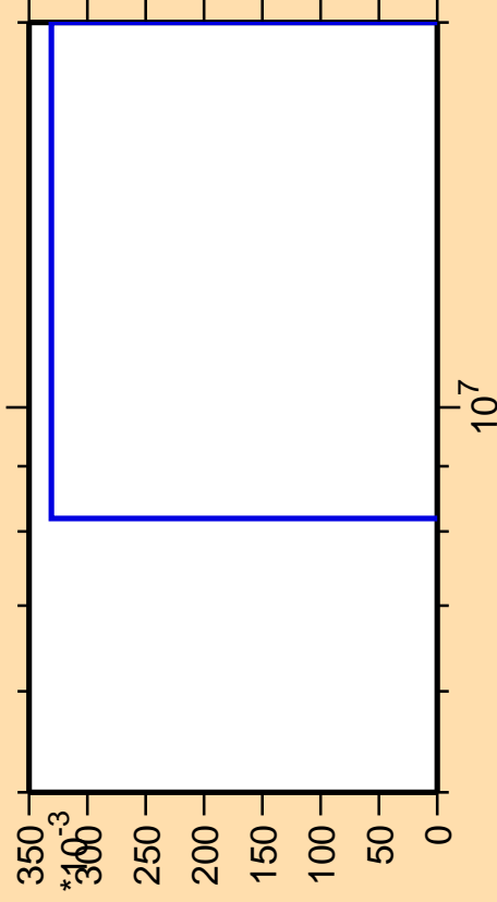
\Delta\sigma/\sigma vs. E for ^{241}\text{Am}(\text{mt117})
