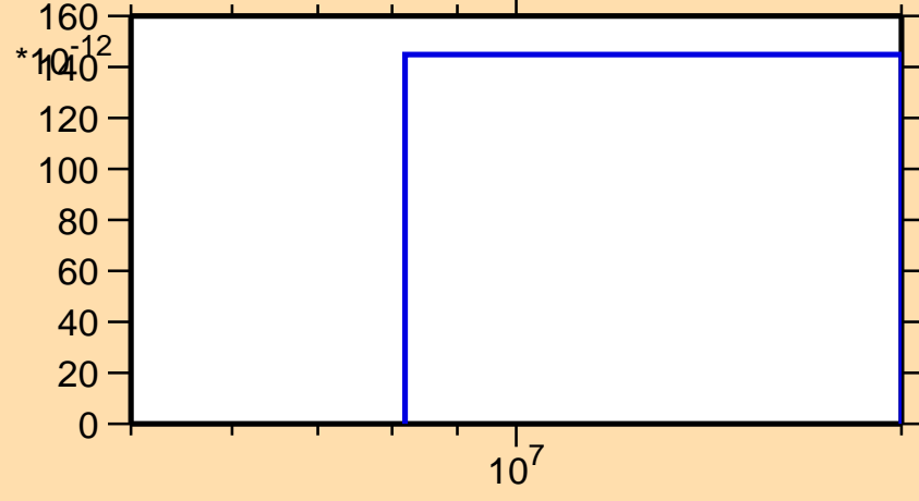
\sigma vs. E for ^{241}\text{Am}(n,p\alpha)
