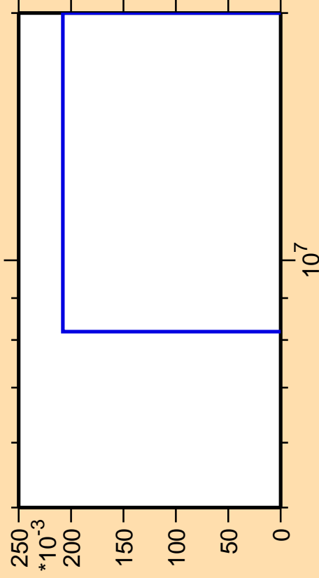
\Delta\sigma/\sigma vs. E for ^{241}\text{Am} (mt 45)
