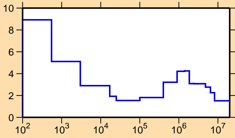
\Delta\sigma/\sigma vs. E for ^{241}\text{Am}(n,\text{el.})
