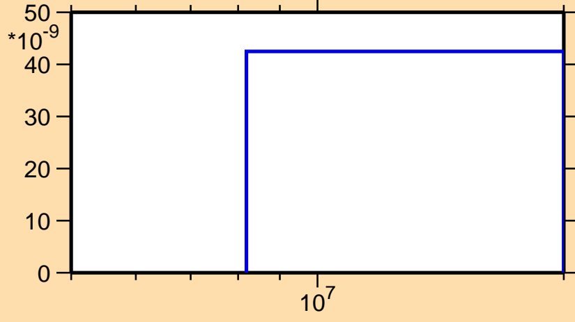
\sigma vs. E for ^{241}\text{Am}(n,nt)
