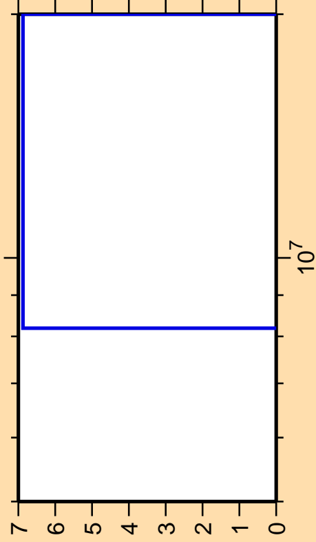
\Delta\sigma/\sigma vs. E for ^{241}\text{Am}(n,\text{nd})
