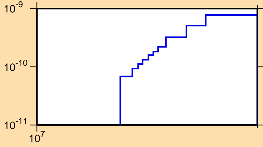
\sigma vs. E for ^{242}\text{Am}(n,p\alpha)
