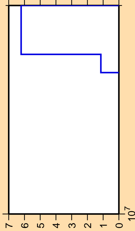
\Delta\sigma/\sigma vs. E for ^{242}\text{Am}(n,\text{He3})
