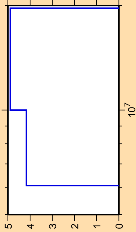
\Delta\sigma/\sigma vs. E for ^{242}\text{Am}(n,t)
