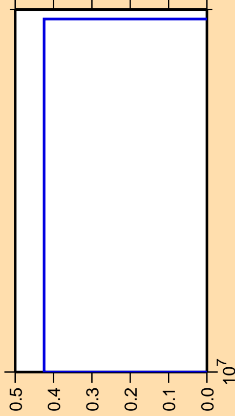
\Delta\sigma/\sigma vs. E for ^{242}\text{Am}(\text{mt117})
