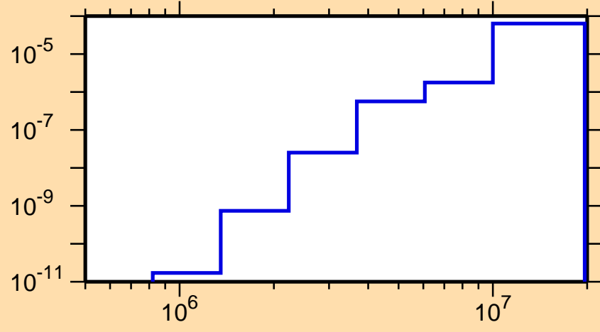
\sigma vs. E for ^{242}\text{Am}(n,n\alpha)
