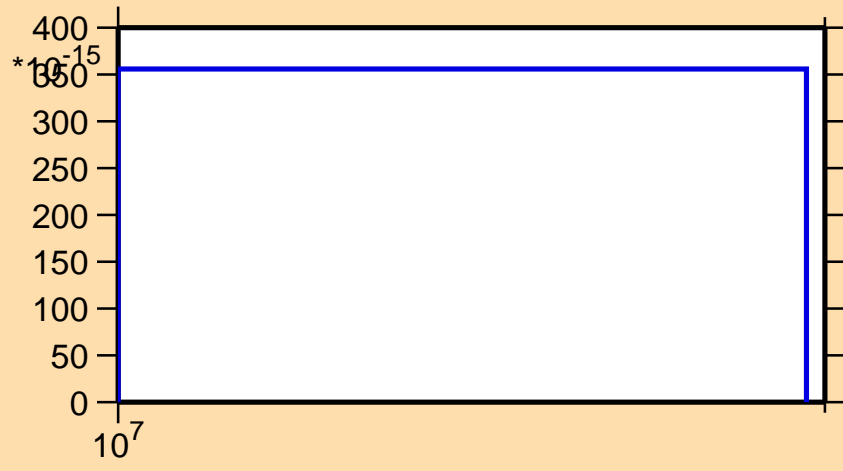
\sigma vs. E for ^{242}\text{Am} (mt 45)
