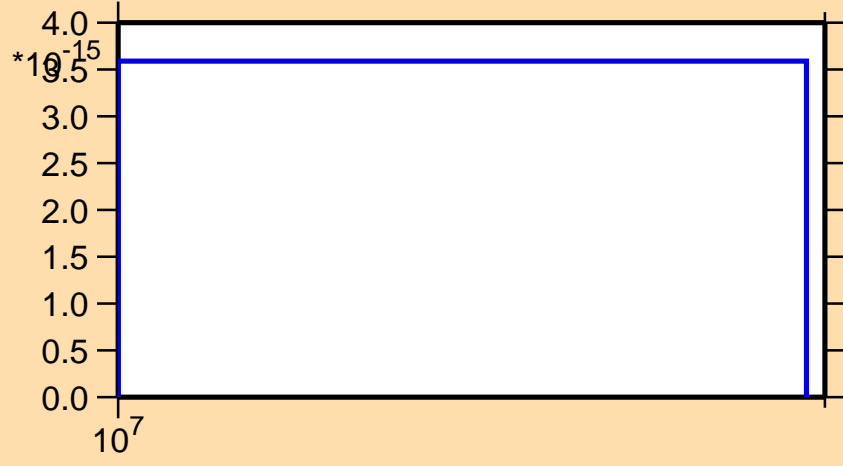
\sigma vs. E for ^{242}\text{Am} (mt 11)
