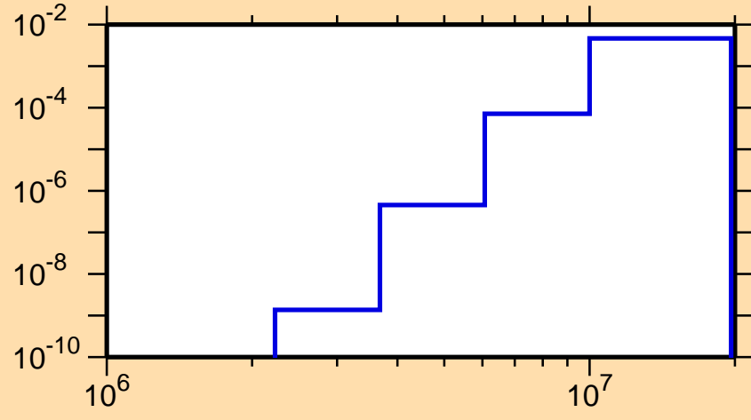
\sigma vs. E for ^{242}\text{Am}(n,p)
