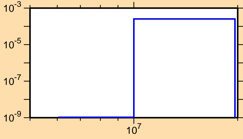
\sigma vs. E for ^{242}\text{Am}(n,d)
