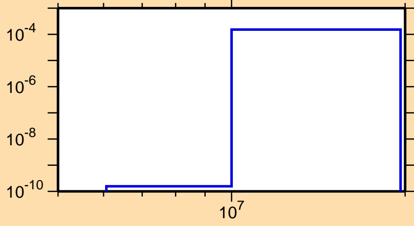
\sigma vs. E for ^{242}\text{Am}(n,np)
