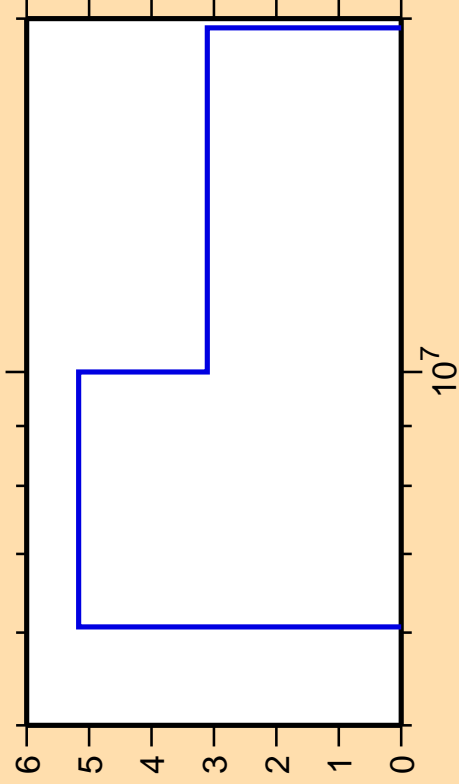
\Delta\sigma/\sigma vs. E for ^{242}\text{Am}(n,d)
