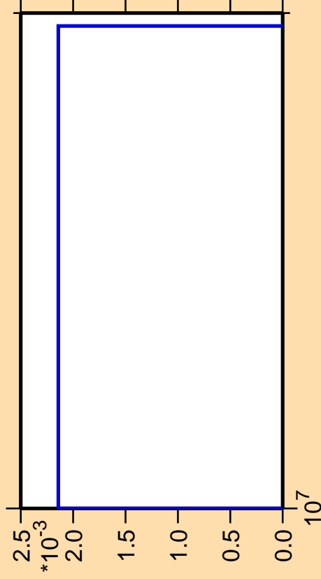
\Delta\sigma/\sigma vs. E for ^{242}\text{Am} (mt 11)
