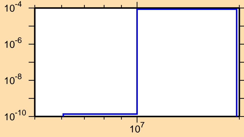
\sigma vs. E for ^{242}\text{Am}(n,t)
