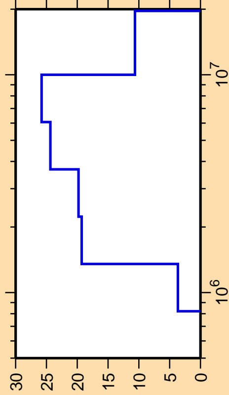
\Delta\sigma/\sigma vs. E for ^{242}\text{Am}(n,n\alpha)
