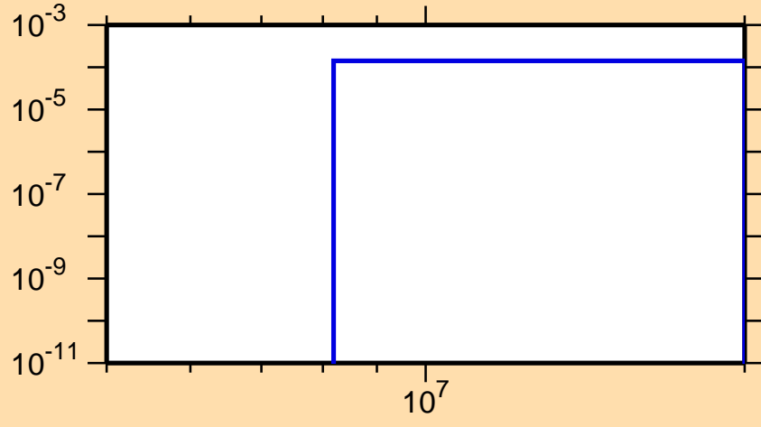
\sigma vs. E for ^{243}\text{Am}(n,d)
