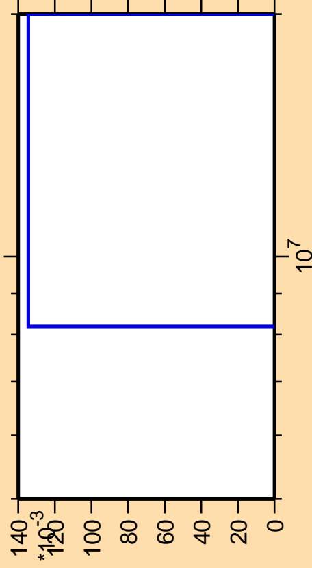
\Delta\sigma/\sigma vs. E for ^{243}\text{Am}(\text{mt117})
