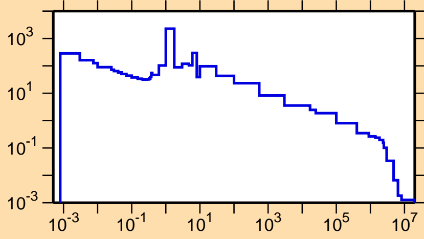
\sigma vs. E for ^{243}\text{Am}(n,\gamma)
