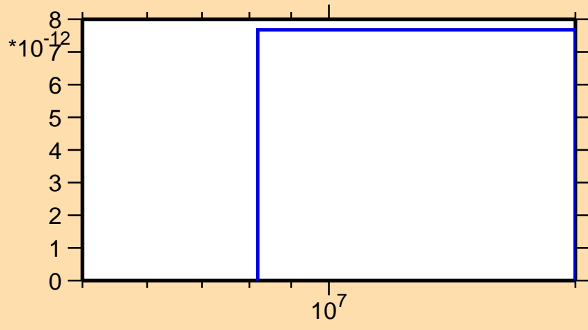
\sigma vs. E for ^{243}\text{Am}(n,p\alpha)
