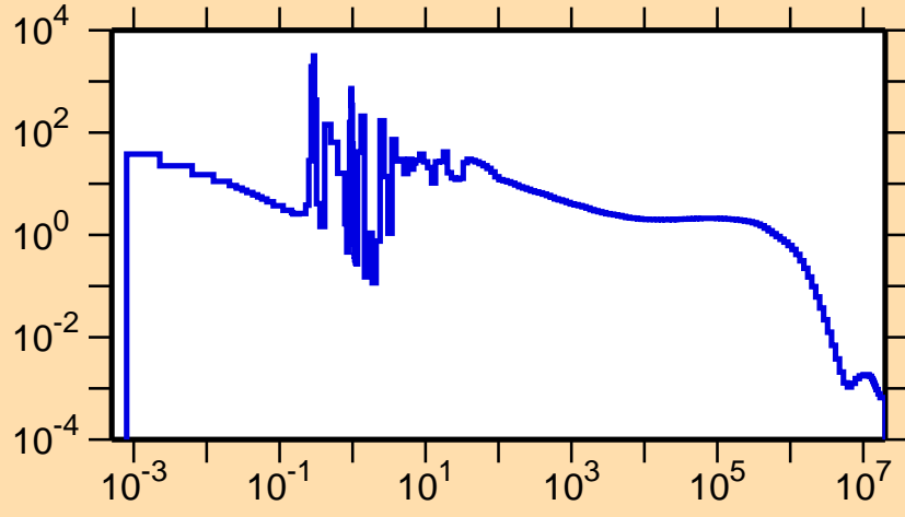
\sigma vs. E for ^{244}\text{Am}(n,\gamma)
