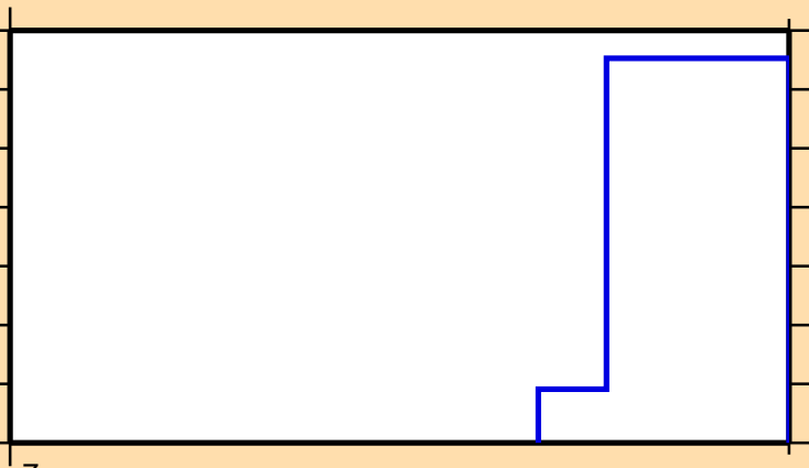
\sigma vs. E for ^{244}\text{Am} (mt 45)
