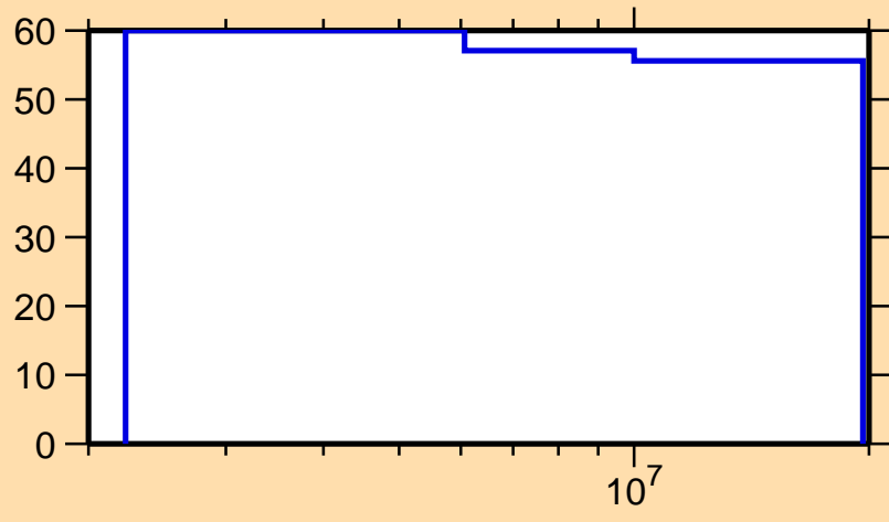
\Delta\sigma/\sigma vs. E for ^{244}\text{Am}(n,p)
