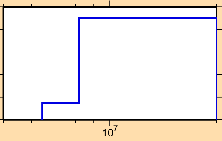
\sigma vs. E for ^{244}\text{Am}(n,2n\alpha)
