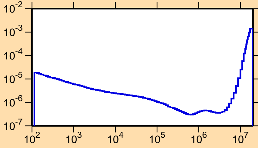
\sigma vs. E for ^{244}\text{Am}(n,\alpha)
