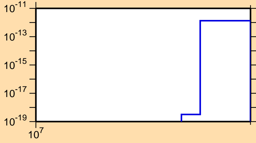
\sigma vs. E for ^{244}\text{Am} (mt 11)
