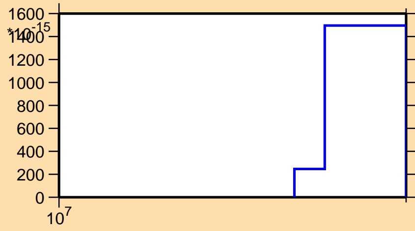
\sigma vs. E for ^{244}\text{Am} (mt 45)
