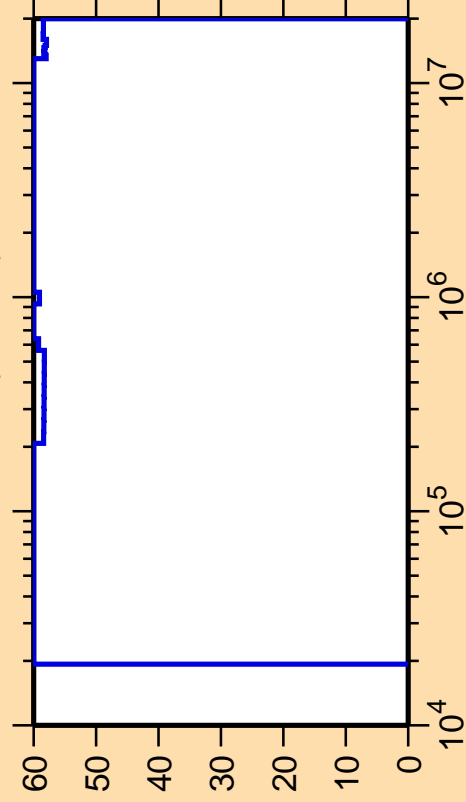
\Delta\sigma/\sigma vs. E for ^{245}\text{Am}(n,\text{inel.})
