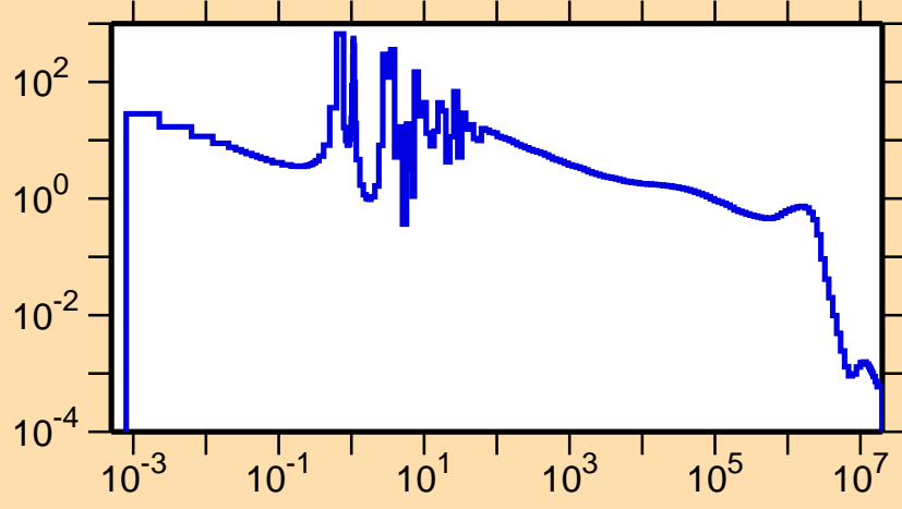
\sigma vs. E for ^{245}\text{Am}(n,\gamma)
