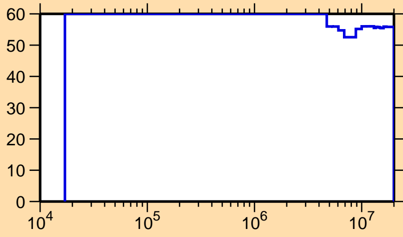
\Delta\sigma/\sigma vs. E for ^{245}\text{Am}(n,n_1)
