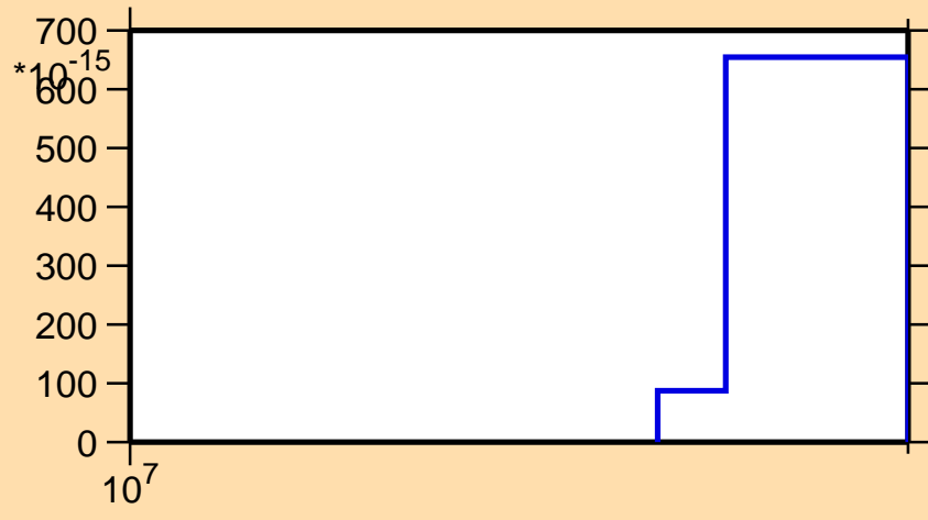
\sigma vs. E for ^{245}\text{Am} (mt 45)
