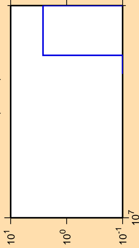
\Delta\sigma/\sigma vs. E for ^{245}\text{Am} (mt 11)
