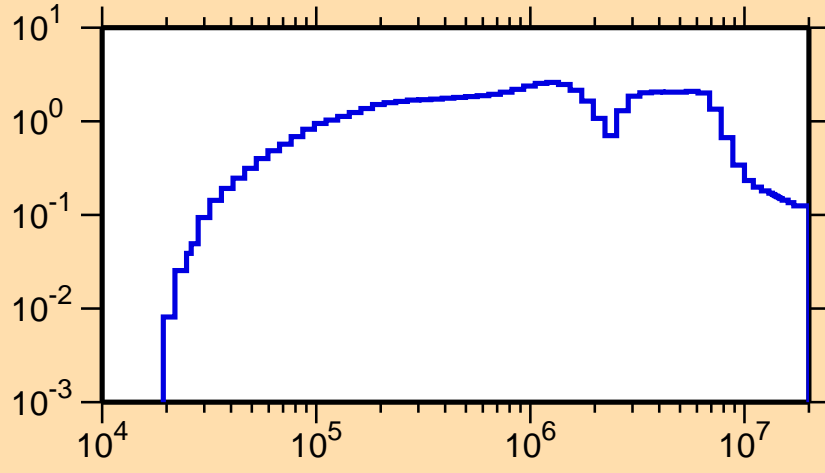
\sigma vs. E for ^{245}\text{Am}(n,\text{inel.})
