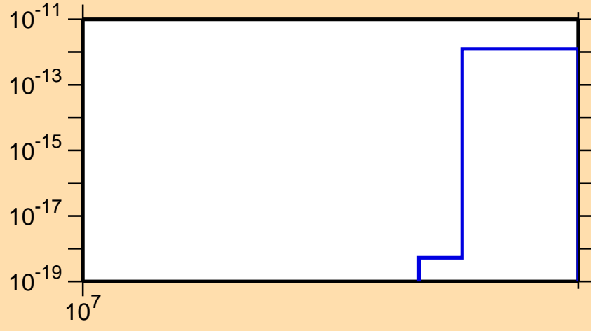
\sigma vs. E for ^{245}\text{Am} (mt 11)
