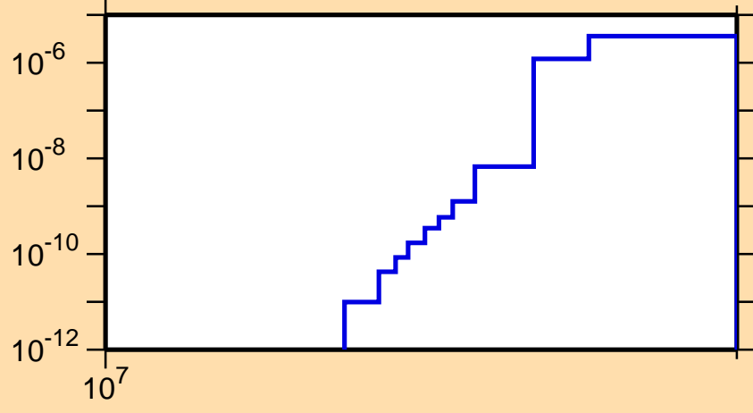
\sigma vs. E for ^{245}\text{Am}(n,3n\alpha)
