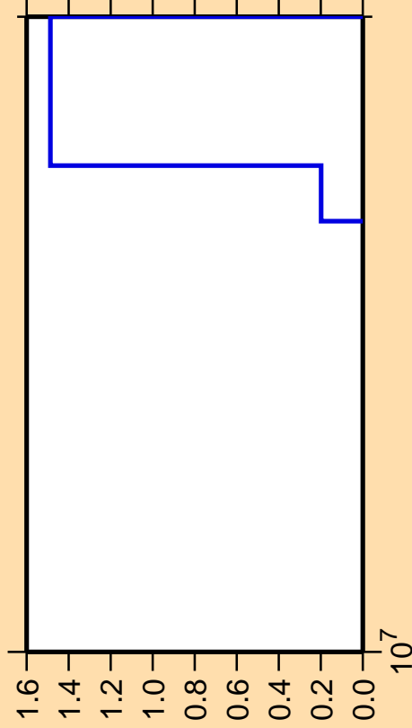
\Delta\sigma/\sigma vs. E for ^{245}\text{Am} (mt 45)
