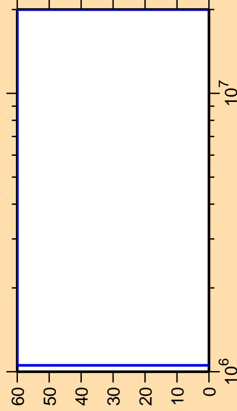
\Delta\sigma/\sigma vs. E for ^{245}\text{Am}(n,n\text{cont.})
