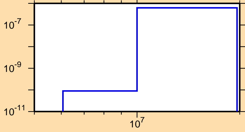
\sigma vs. E for ^{245}\text{Am}(n,2n\alpha)
