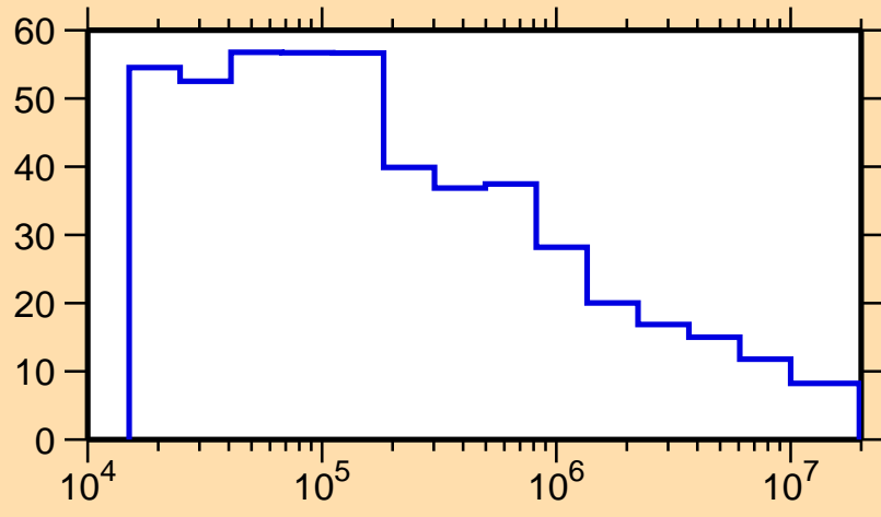
\Delta\sigma/\sigma vs. E for ^{245}\text{Am}(n,\text{nonel.})
