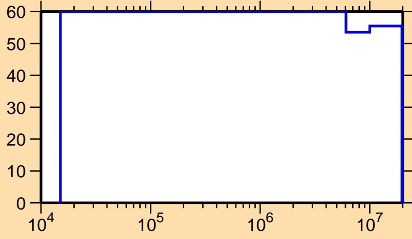
\Delta\sigma/\sigma vs. E for ^{245}\text{Am}(n,n_1)
