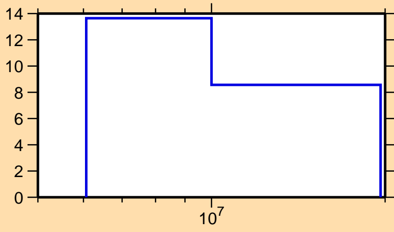
\Delta\sigma/\sigma vs. E for ^{245}\text{Am}(n,\text{el.})
