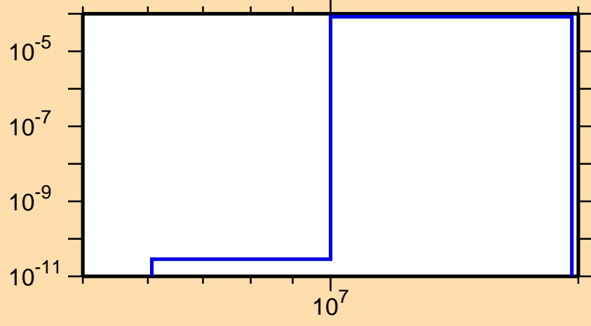
\sigma vs. E for ^{245}\text{Am}(n,np)
