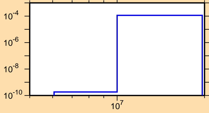
\sigma vs. E for ^{245}\text{Am}(n,d)
