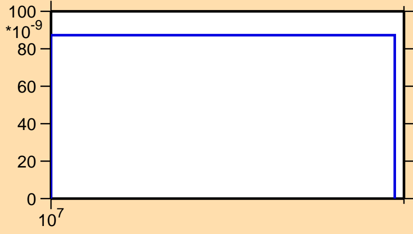
\sigma vs. E for ^{245}\text{Am}(n,3n\alpha)
