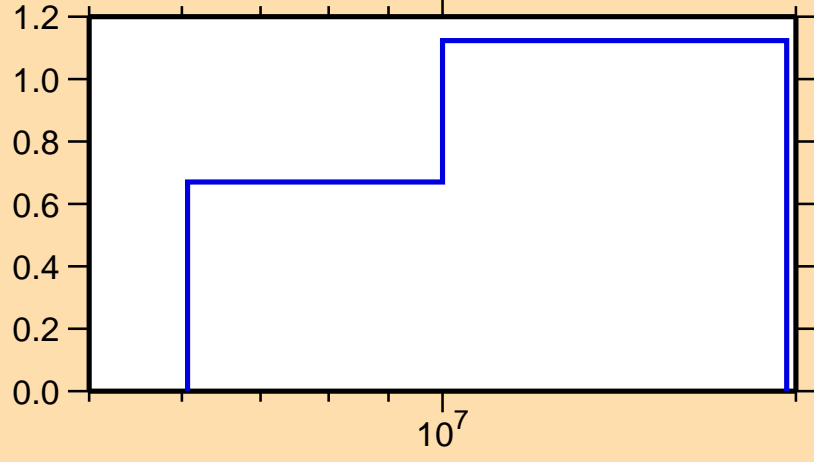
\sigma vs. E for ^{245}\text{Am}(n,2n)
