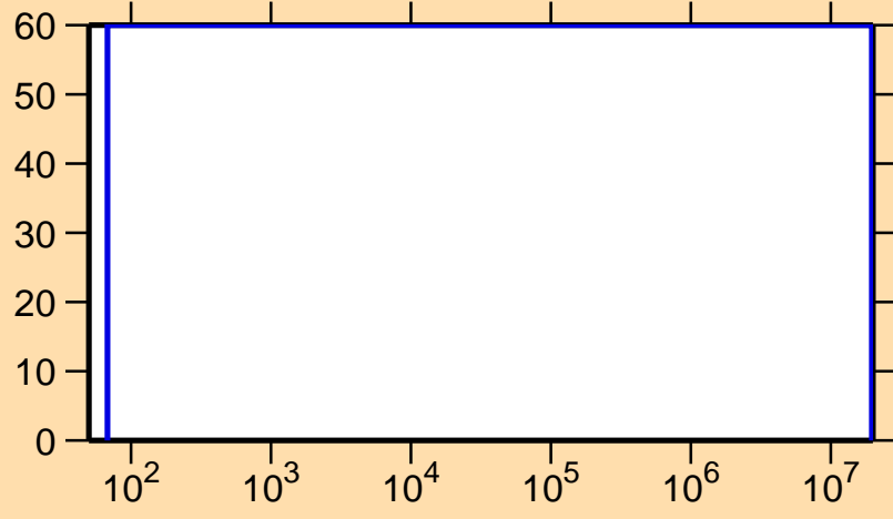
\Delta\sigma/\sigma vs. E for ^{245}\text{Am}(n,f)
