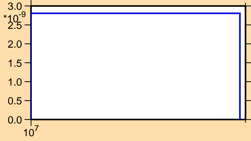
\sigma vs. E for ^{245}\text{Am}(n,2np)
