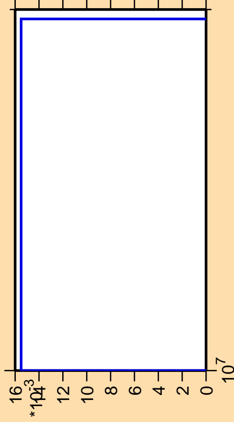
\Delta\sigma/\sigma vs. E for ^{245}\text{Am} (mt 11)
