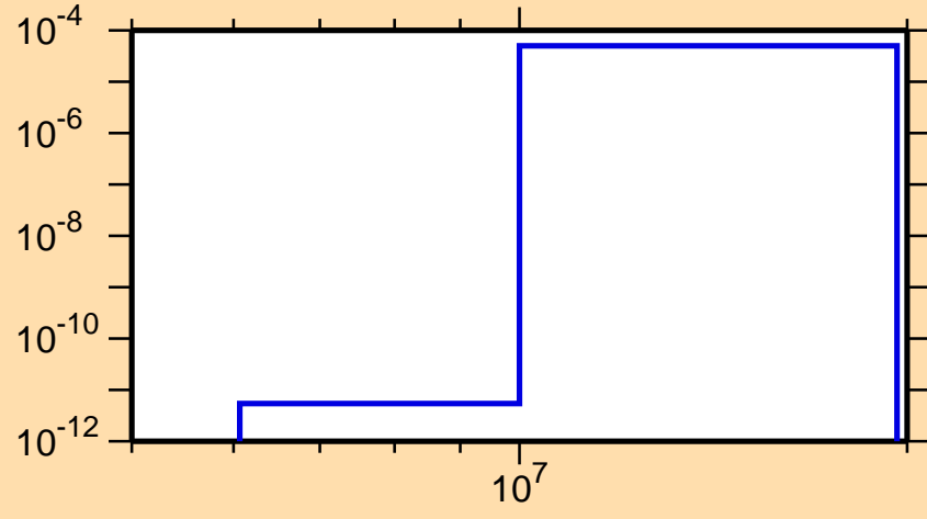
\sigma vs. E for ^{245}\text{Am}(n,t)
