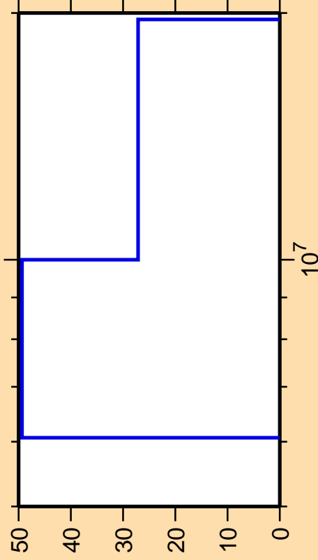
\Delta\sigma/\sigma vs. E for ^{245}\text{Am}(n,d)
