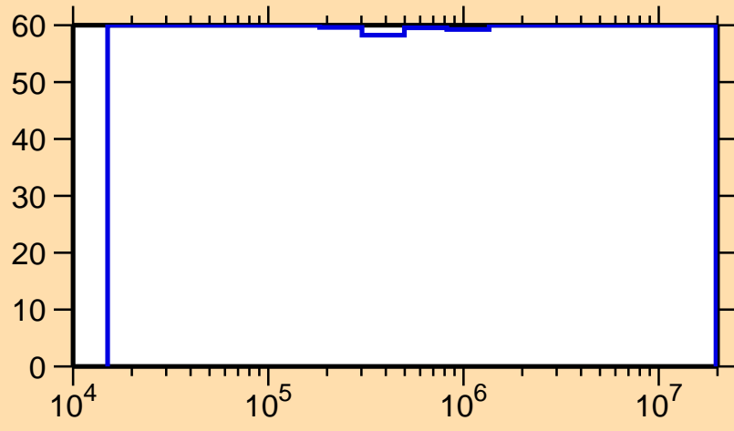
\Delta\sigma/\sigma vs. E for ^{245}\text{Am}(n,\text{inel.})
