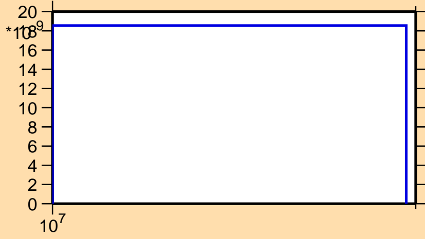
\sigma vs. E for ^{245}\text{Am}(n,\text{nd})
