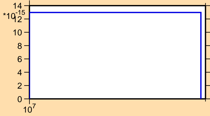
\sigma vs. E for ^{245}\text{Am} (mt 45)
