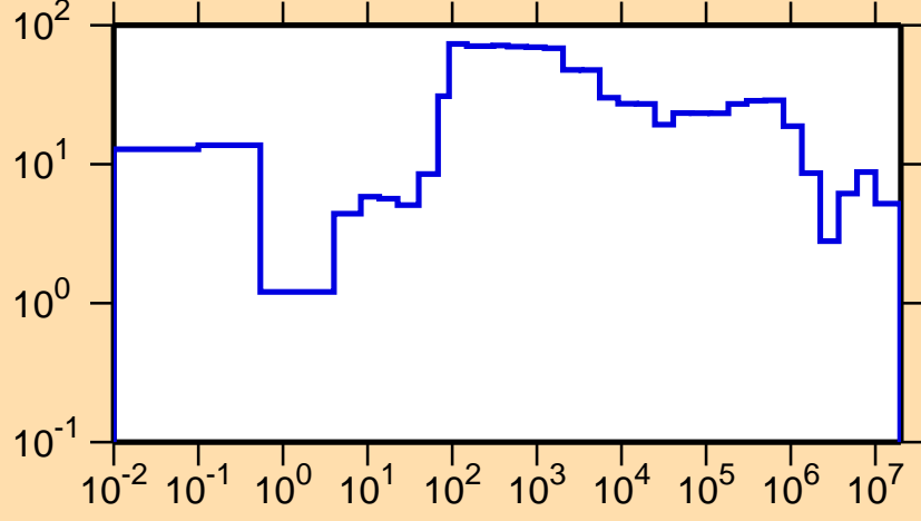
\Delta\sigma/\sigma vs. E for ^{245}\text{Am}(n,\text{tot.})
