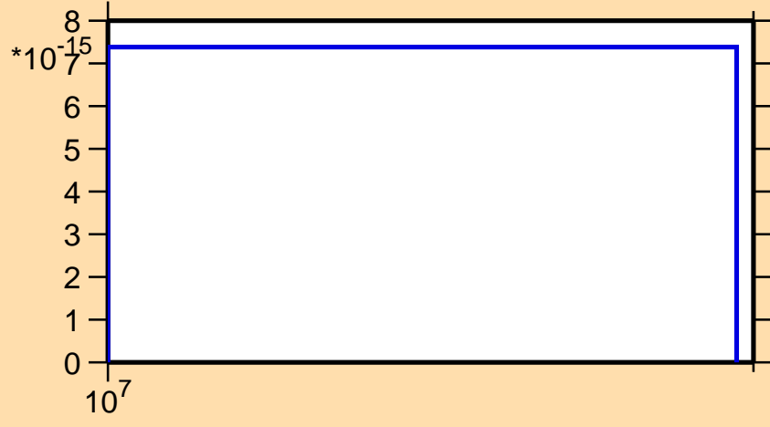
\sigma vs. E for ^{245}\text{Am} (mt 11)
