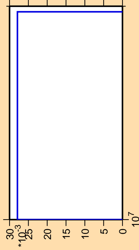
\Delta\sigma/\sigma vs. E for ^{245}\text{Am}(n,\text{He}3)
