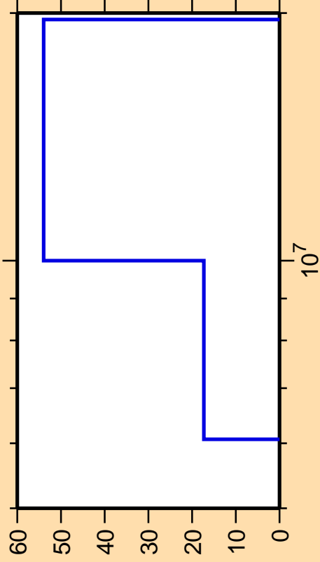
\Delta\sigma/\sigma vs. E for ^{245}\text{Am}(n,np)
