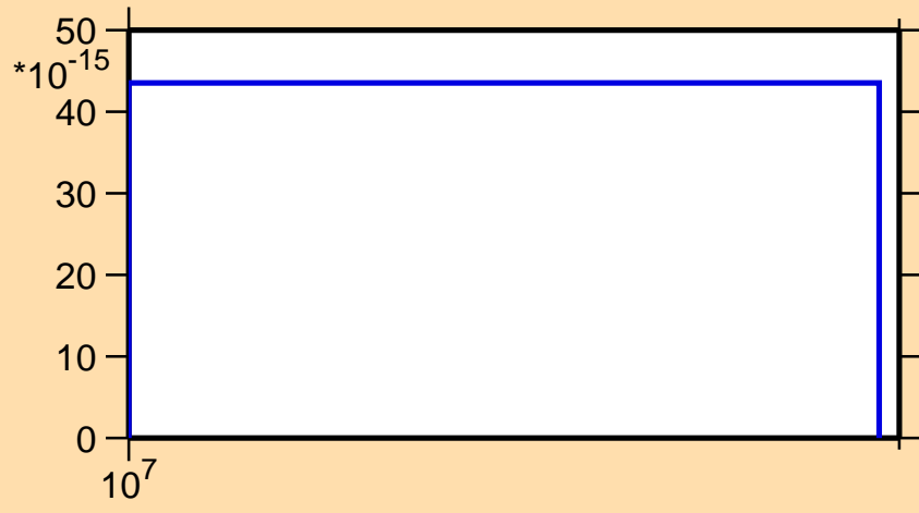
\sigma vs. E for ^{245}\text{Am}(n,\text{He}3)
