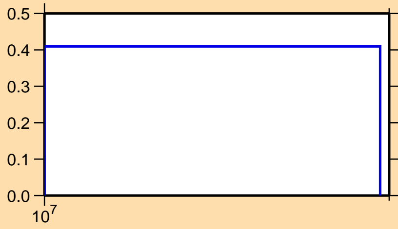
\sigma vs. E for ^{245}\text{Am}(n,3n)
