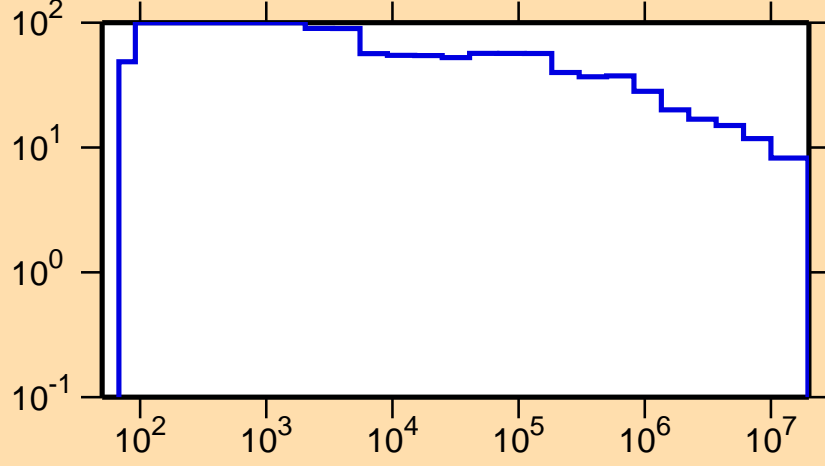
\Delta\sigma/\sigma vs. E for ^{245}\text{Am}(n,\text{nonel.})
