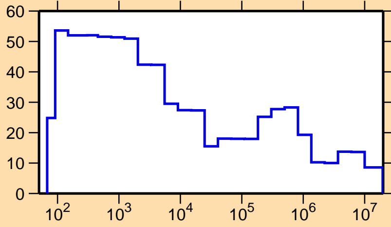
\Delta\sigma/\sigma vs. E for ^{245}\text{Am}(n,\text{el.})
