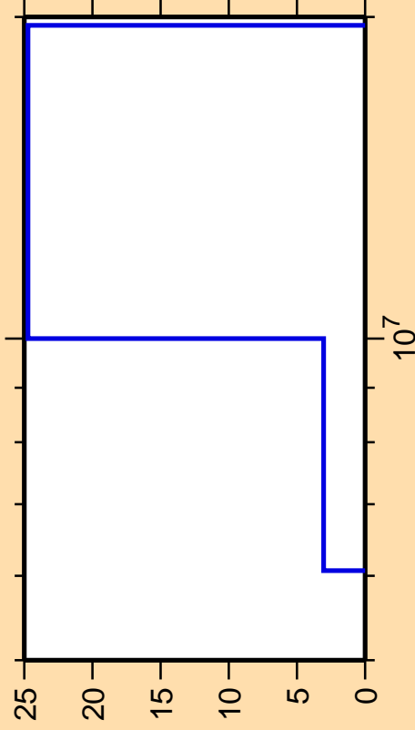
\Delta\sigma/\sigma vs. E for ^{245}\text{Am}(n,t)
