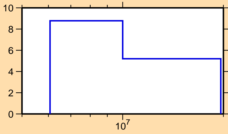
\Delta\sigma/\sigma vs. E for ^{245}\text{Am}(n,\text{tot.})
