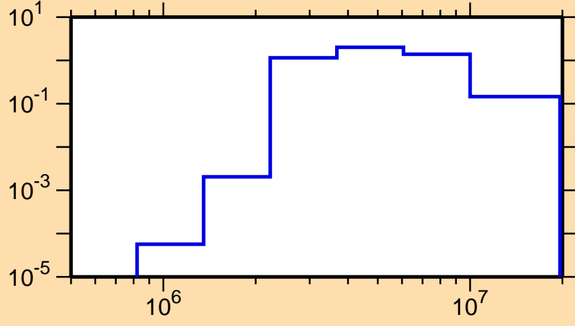
\sigma vs. E for ^{245}\text{Am}(n,n\text{cont.})
