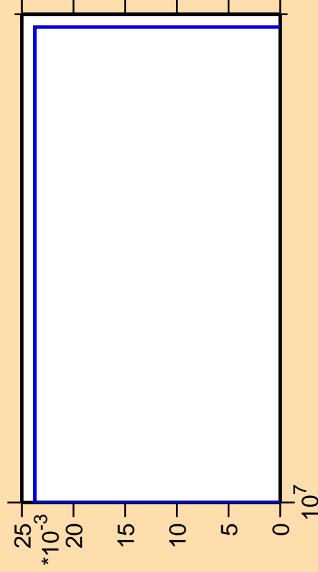
\Delta\sigma/\sigma vs. E for ^{245}\text{Am} (mt 45)
