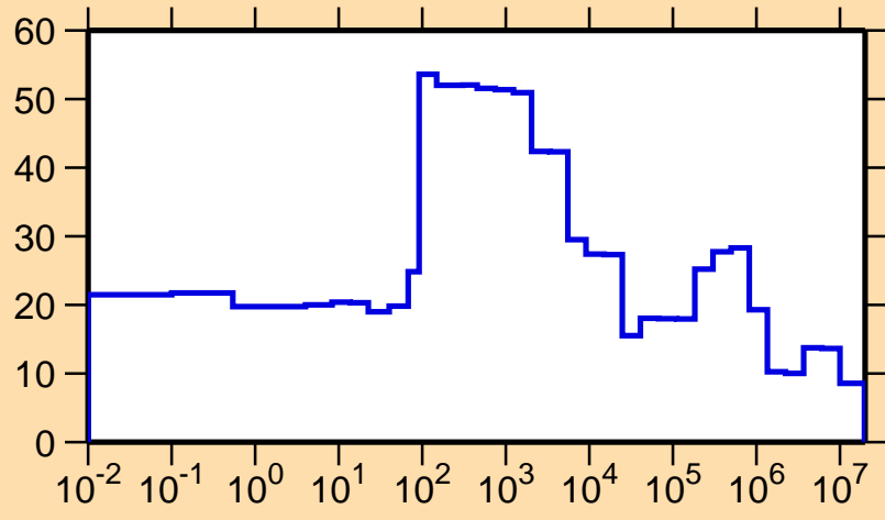
\Delta\sigma/\sigma vs. E for ^{245}\text{Am}(n,el.)
