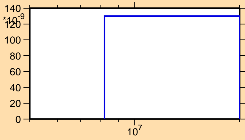
\sigma vs. E for ^{245}\text{Am}(n,nt)
