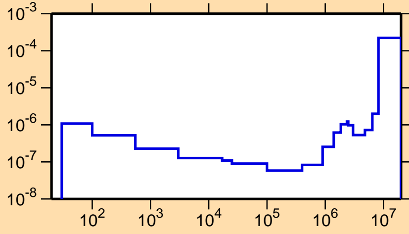
\sigma vs. E for ^{245}\text{Am}(n,\alpha)
