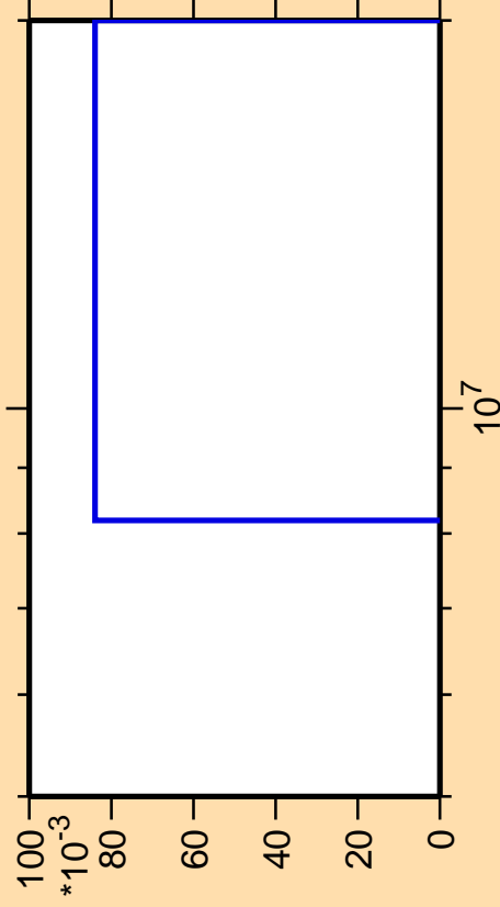
\Delta\sigma/\sigma vs. E for ^{246}\text{Am}(n,\text{He3})
