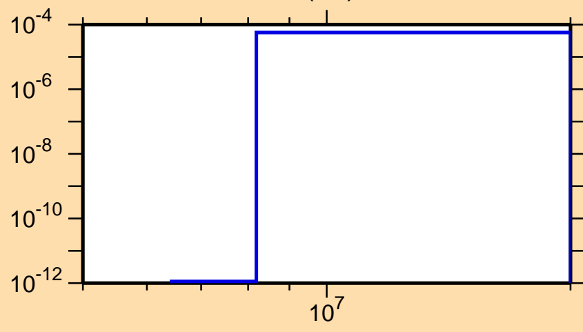
\sigma vs. E for ^{246}\text{Am}(n,t)
