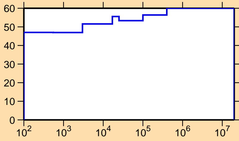
\Delta\sigma/\sigma vs. E for ^{246}\text{Am}(n,\gamma)
