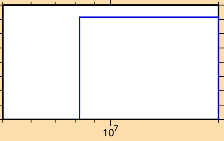
\sigma vs. E for ^{246}\text{Am}(n,\text{He3})
