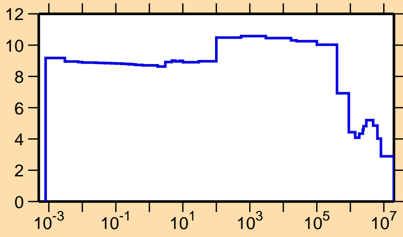
\sigma vs. E for ^{246}\text{Am}(n,\text{el.})
