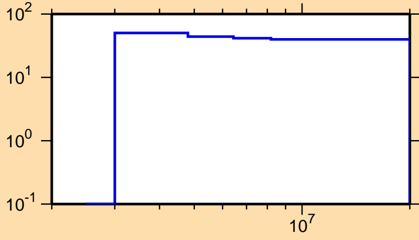
\Delta\sigma/\sigma vs. E for ^{246}\text{Am}(n,p)
