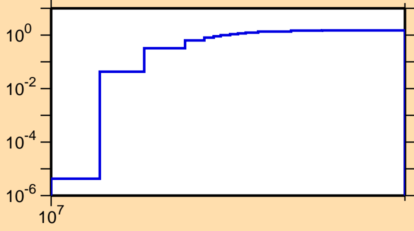
\sigma vs. E for ^{246}\text{Am}(n,3n)
