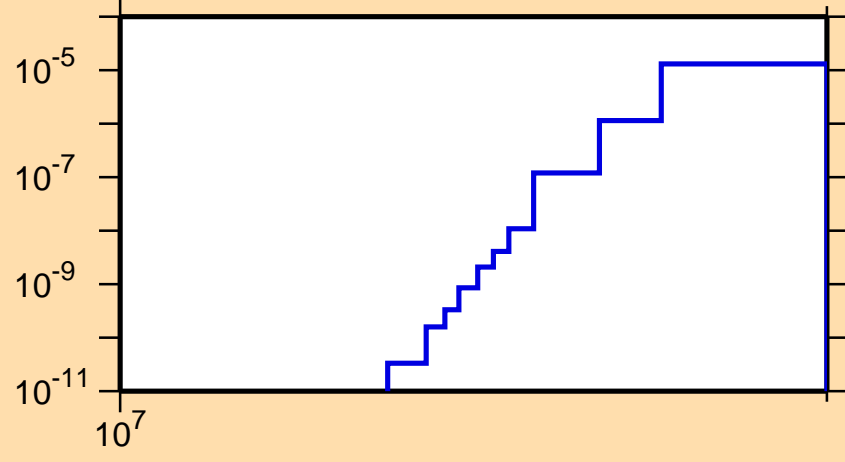
\sigma vs. E for ^{246}\text{Am}(n,nt)
