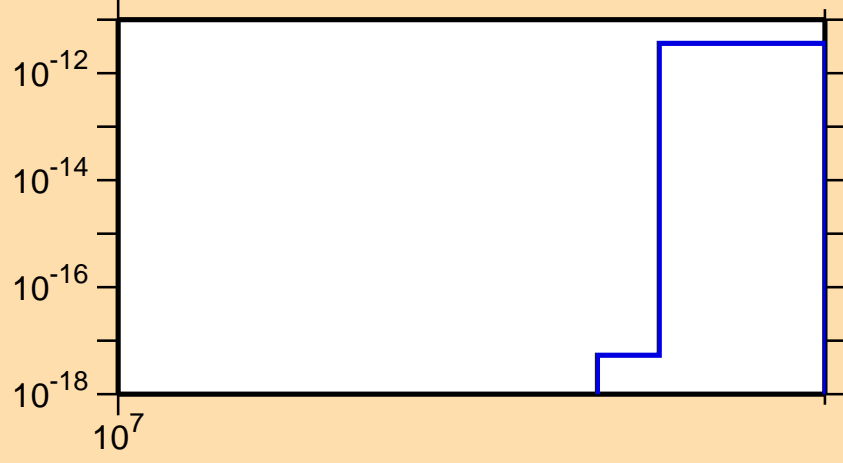
\sigma vs. E for ^{246}\text{Am} (mt 11)
