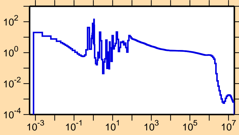
\sigma vs. E for ^{246}\text{Am}(n,\gamma)
