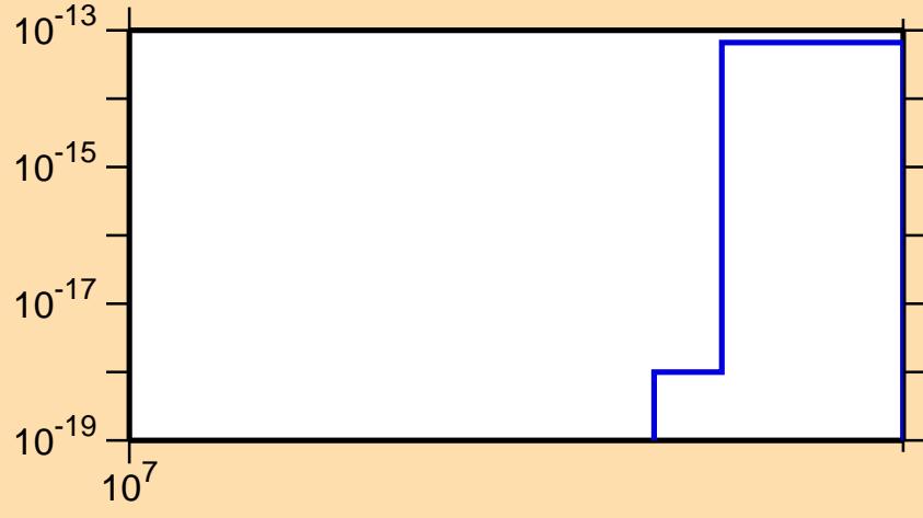
\sigma vs. E for ^{246}\text{Am} (mt 42)
