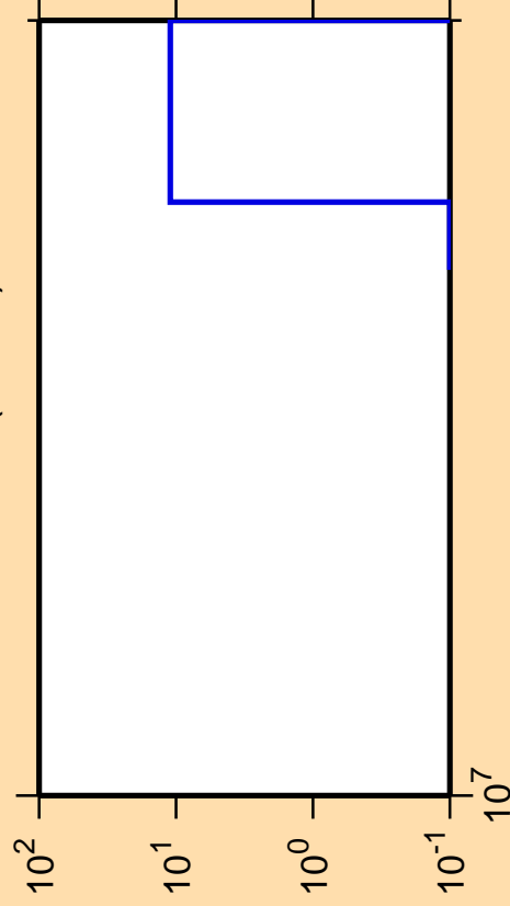
\Delta\sigma/\sigma vs. E for ^{246}\text{Am} (mt 11)
