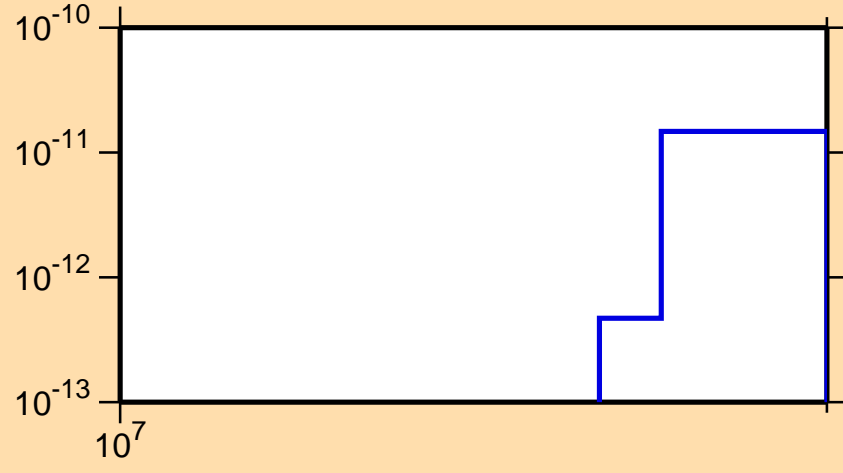
\sigma vs. E for ^{246}\text{Am}(n,\text{He3})
