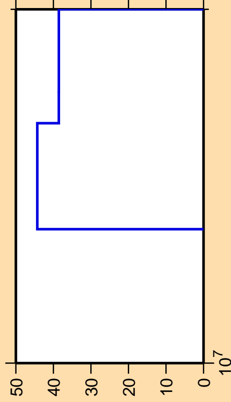
\Delta\sigma/\sigma vs. E for ^{246}\text{Am}(n,nd)
