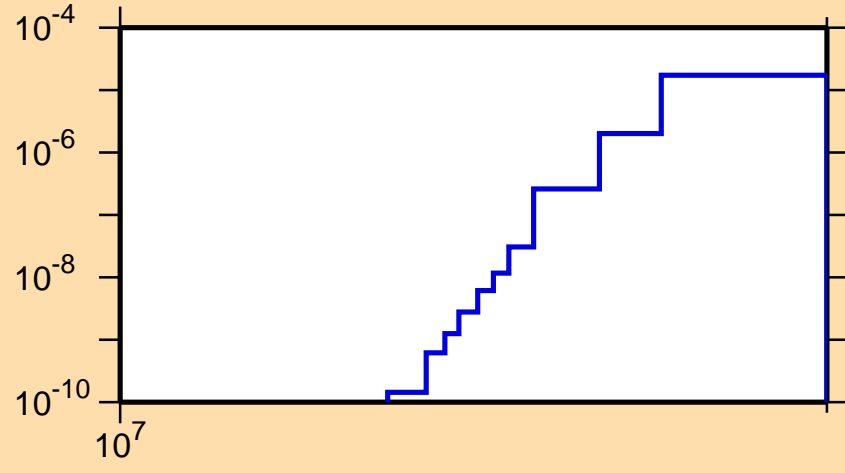
\sigma vs. E for ^{246}\text{Am}(n,nd)
