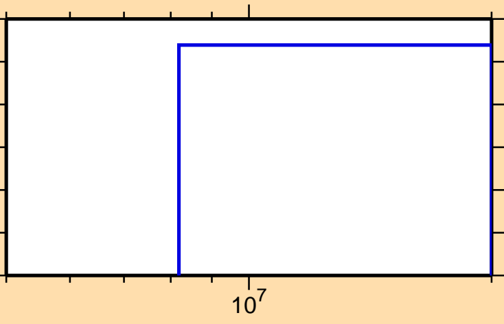
\sigma vs. E for ^{246}\text{Am} (mt 42)
