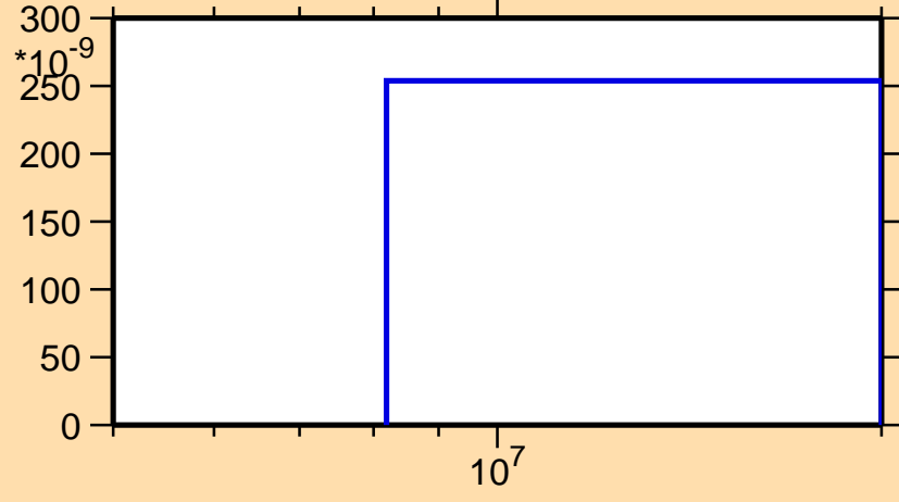
\sigma vs. E for ^{246}\text{Am}(n,\text{nd})
