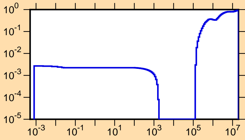
\mu vs. E for ^{247}\text{Am}(\text{mt251})
