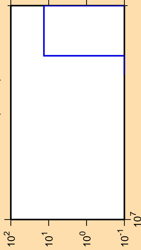
\Delta\sigma/\sigma vs. E for ^{247}\text{Am} (mt 11)
