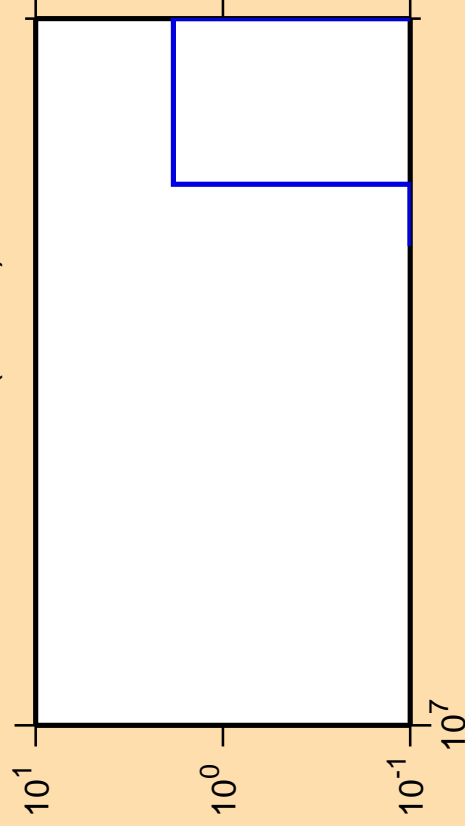
\Delta\sigma/\sigma vs. E for ^{247}\text{Am} (mt 42)
