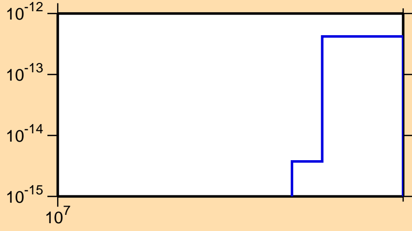
\sigma vs. E for ^{247}\text{Am}(n,\text{He3})
