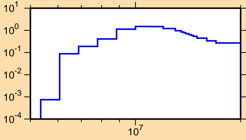
\sigma vs. E for ^{247}\text{Am}(n,2n)
