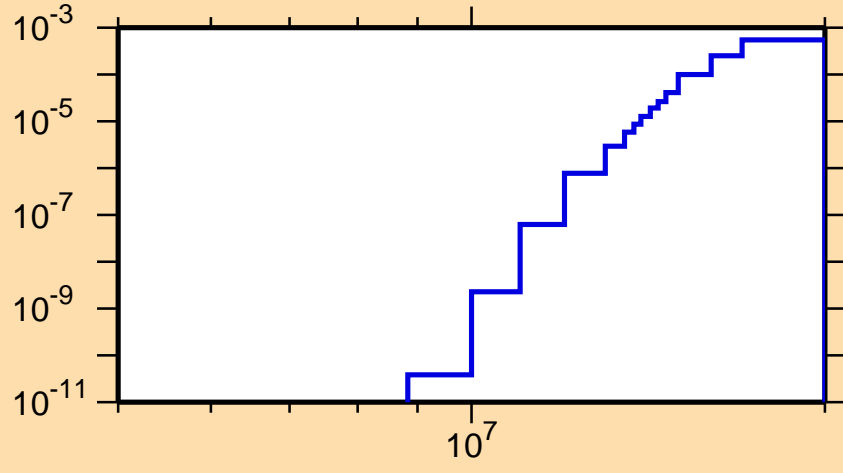
\sigma vs. E for ^{247}\text{Am}(n,t)
