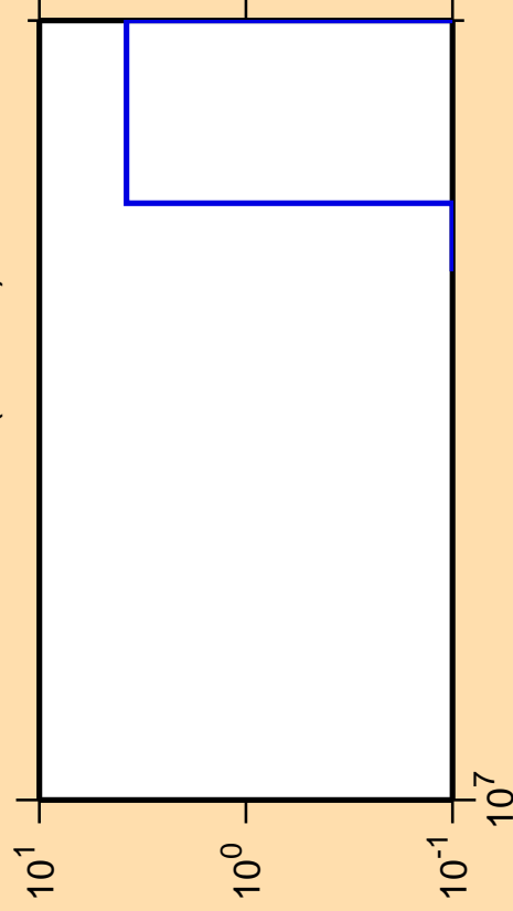
\Delta\sigma/\sigma vs. E for ^{247}\text{Am}(n,\text{He3})
