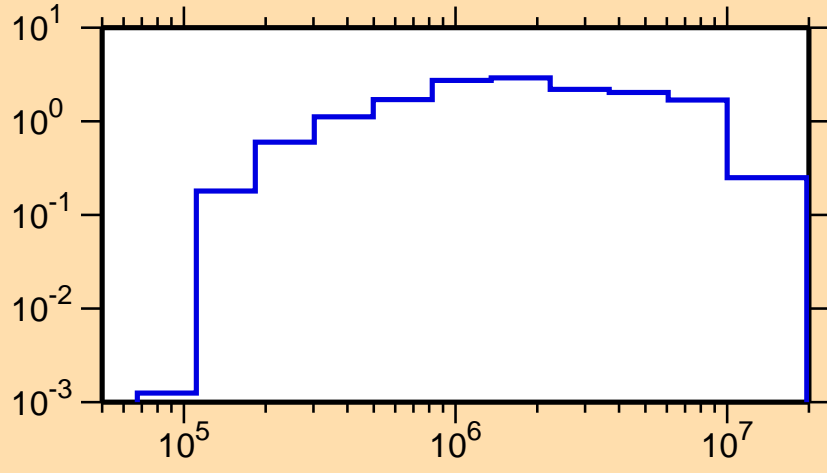
\sigma vs. E for ^{247}\text{Am}(n,\text{inel.})
