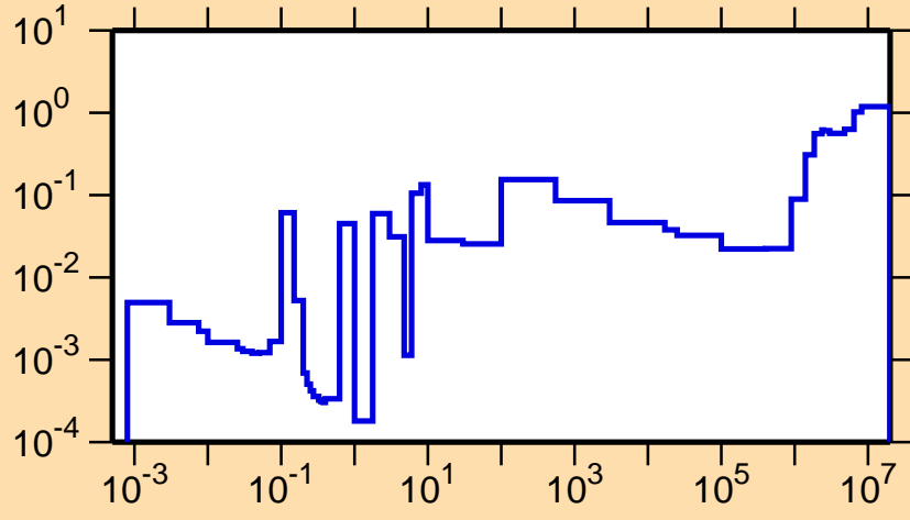
\sigma vs. E for ^{247}\text{Am}(n,f)
