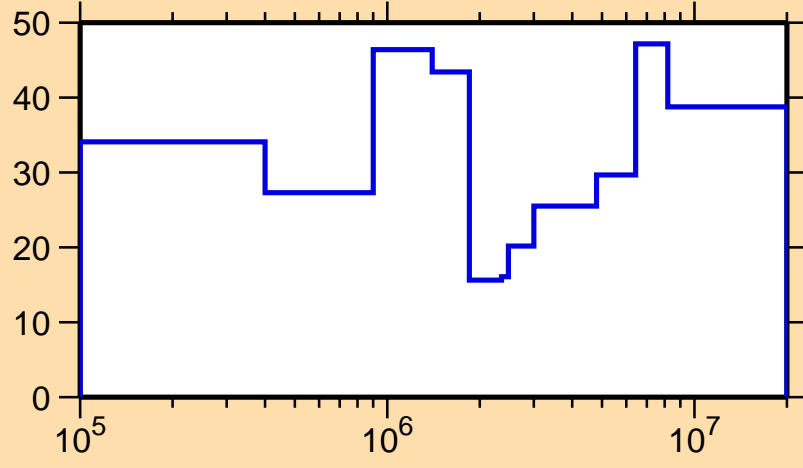
\Delta\sigma/\sigma vs. E for ^{247}\text{Am}(n, el.)
