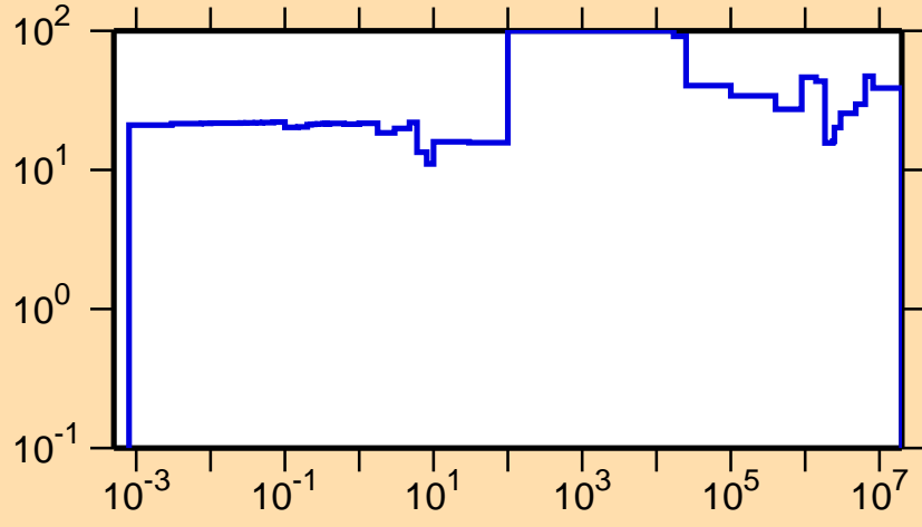
\Delta\sigma/\sigma vs. E for ^{247}\text{Am}(n,el.)
