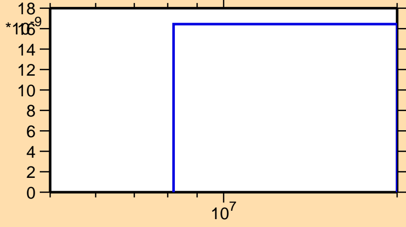
\sigma vs. E for ^{247}\text{Am}(n,\text{nd})
