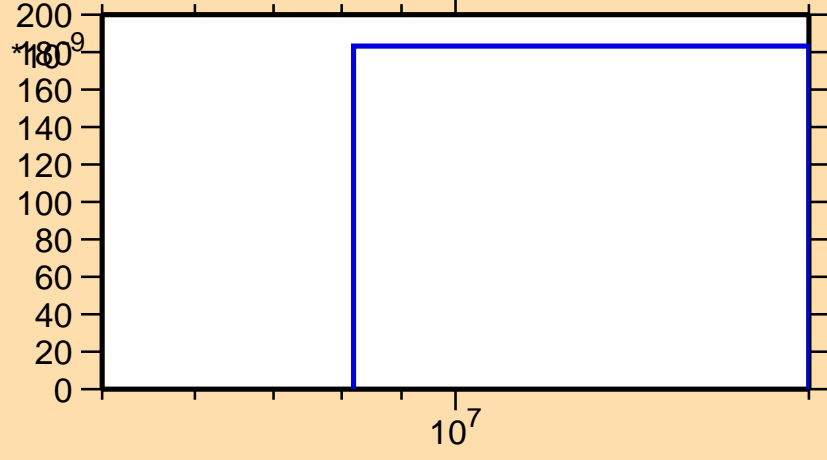
\sigma vs. E for ^{247}\text{Am}(n,nt)
