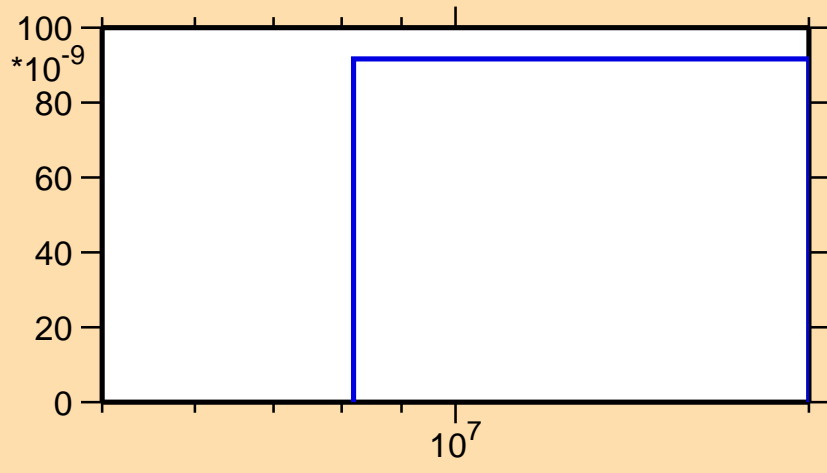
\sigma vs. E for ^{247}\text{Am}(n,3n\alpha)
