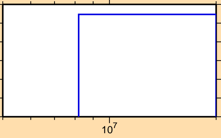
\sigma vs. E for ^{247}\text{Am}(n,np)
