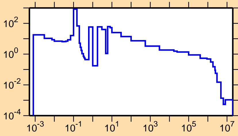
\sigma vs. E for ^{247}\text{Am}(n,\gamma)
