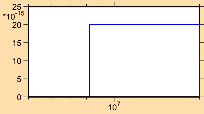
\sigma vs. E for ^{247}\text{Am} (mt 11)
