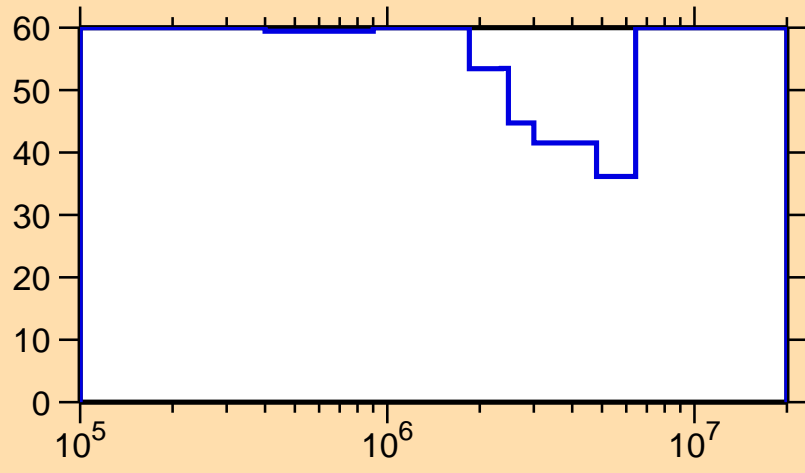
\Delta\sigma/\sigma vs. E for ^{247}\text{Am}(n,\text{inel.})
