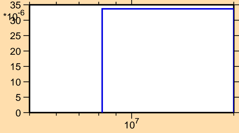
\sigma vs. E for ^{247}\text{Am}(n,t)
