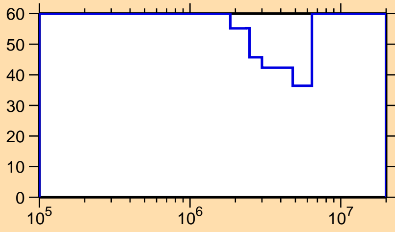
\Delta\sigma/\sigma vs. E for ^{247}\text{Am}(n,n\text{cont.})
