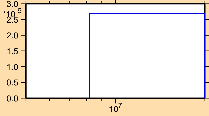
\sigma vs. E for ^{247}\text{Am}(n,2np)
