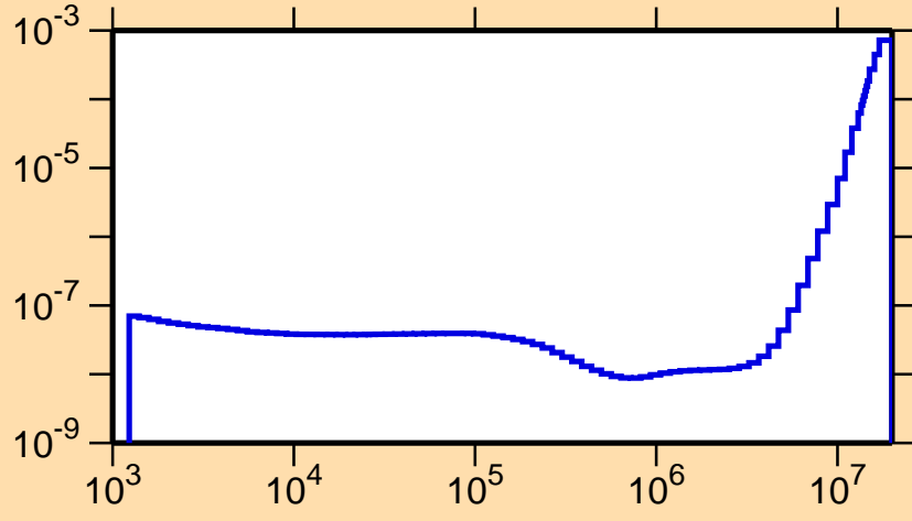
\sigma vs. E for ^{248}\text{Am}(n,\alpha)
