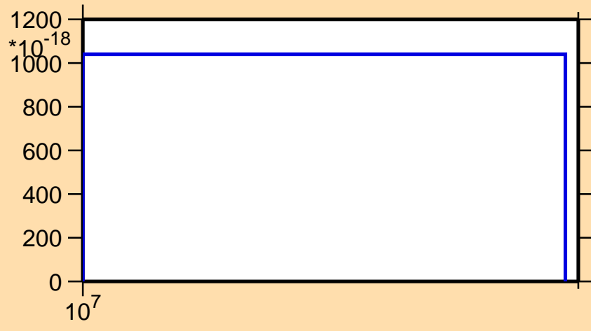
\sigma vs. E for ^{248}\text{Am} (mt 42)
