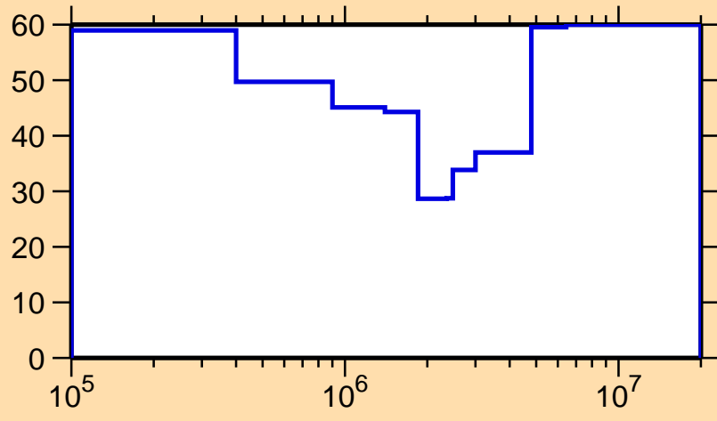
\Delta\sigma/\sigma vs. E for ^{248}\text{Am}(n,n\text{cont.})
