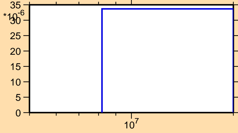
\sigma vs. E for ^{248}\text{Am}(n,np)
