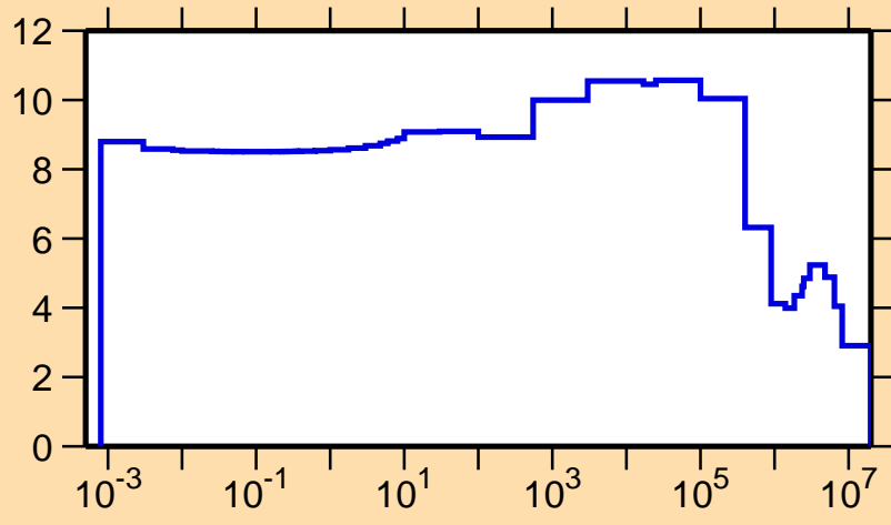
\sigma vs. E for ^{248}\text{Am}(n,\text{el.})
