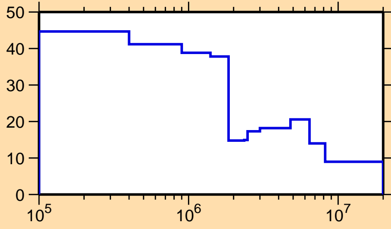
\Delta\sigma/\sigma vs. E for ^{248}\text{Am}(n,\text{nonel.})
