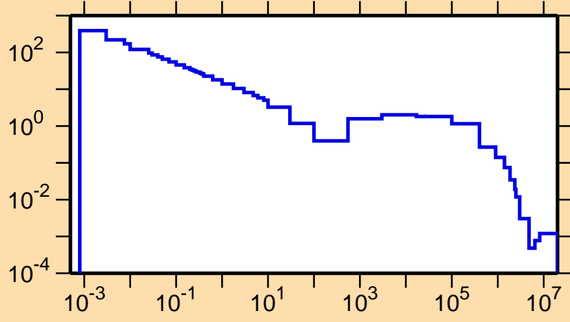
\sigma vs. E for ^{248}\text{Am}(n,\gamma)
