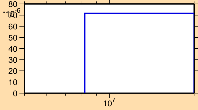
\sigma vs. E for ^{248}\text{Am}(n,3n\alpha)
