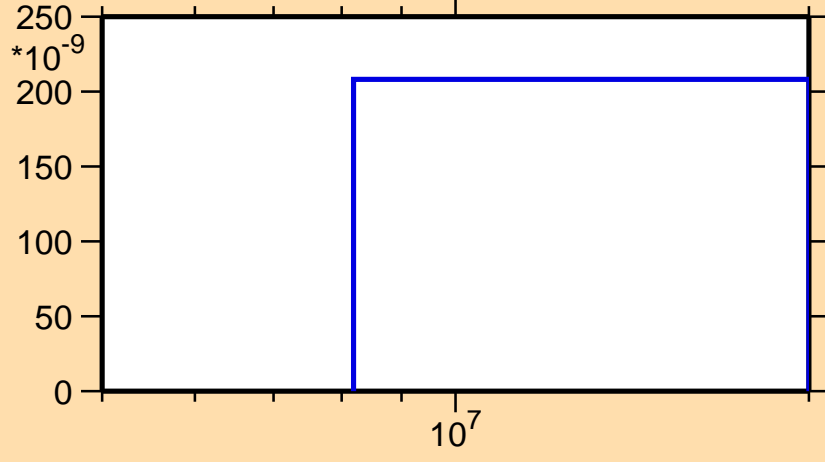
\sigma vs. E for ^{248}\text{Am}(n,nt)
