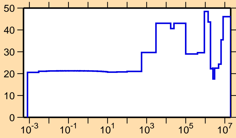
\Delta\sigma/\sigma vs. E for ^{248}\text{Am}(n,el.)
