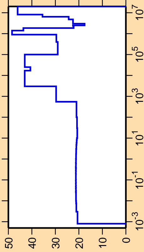
\Delta\sigma/\sigma vs. E for ^{248}\text{Am}(n,\text{el.})
