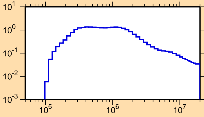
\sigma vs. E for ^{249}\text{Am}(n,n_1)
