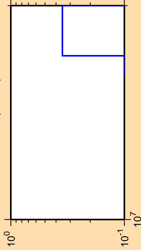
\Delta\sigma/\sigma vs. E for ^{249}\text{Am} (mt 42)
