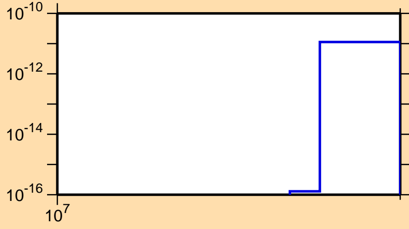
\sigma vs. E for ^{249}\text{Am} (mt 11)
