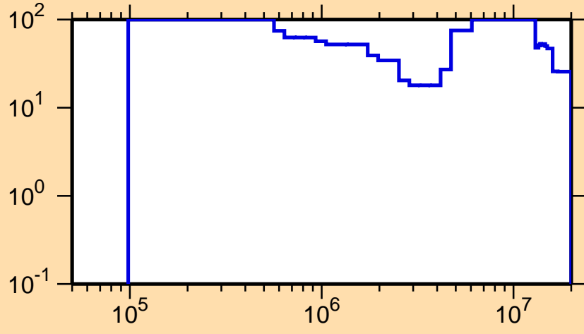
\Delta\sigma/\sigma vs. E for ^{249}\text{Am}(n,n\text{cont.})
