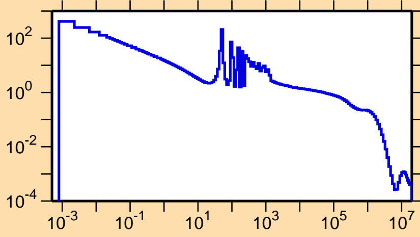
\sigma vs. E for ^{249}\text{Am}(n,\gamma)
