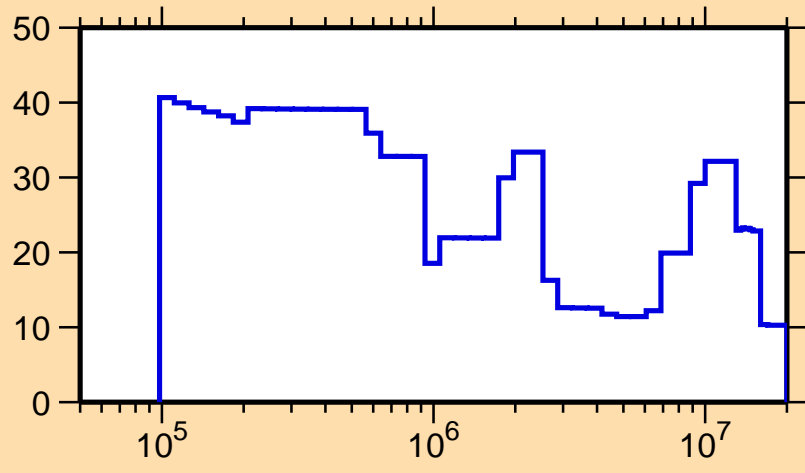
\Delta\sigma/\sigma vs. E for ^{249}\text{Am}(n,\text{tot.})
