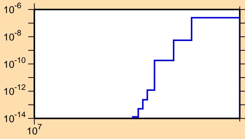
\sigma vs. E for ^{249}\text{Am}(n,2np)
