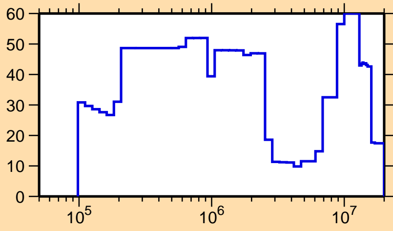
\Delta\sigma/\sigma vs. E for ^{249}\text{Am}(n,\text{el.})
