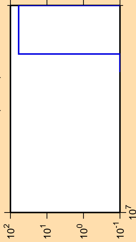
\Delta\sigma/\sigma vs. E for ^{249}\text{Am} (mt 11)
