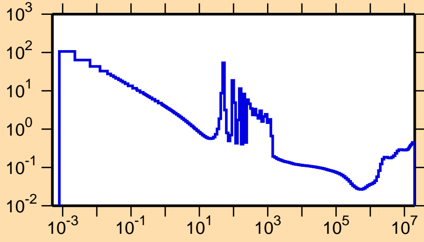
\sigma vs. E for ^{249}\text{Am}(n,f)
