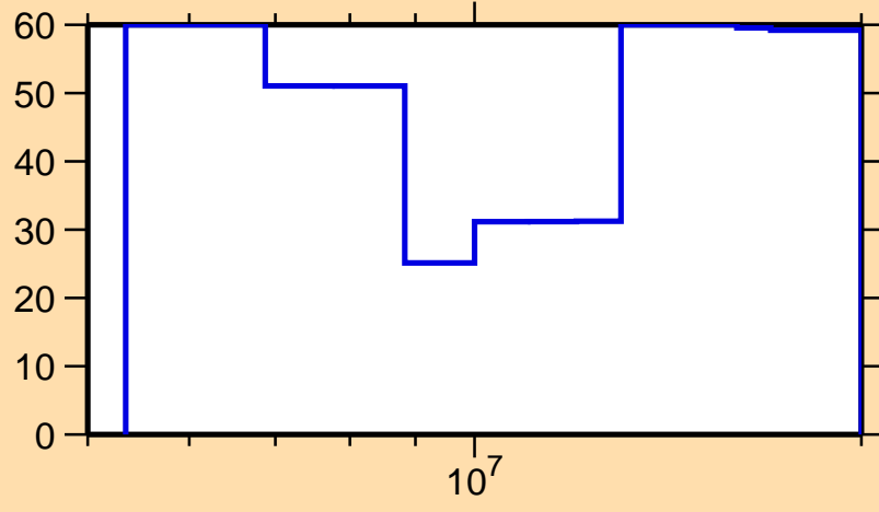
\Delta\sigma/\sigma vs. E for ^{249}\text{Am}(n,2n)
