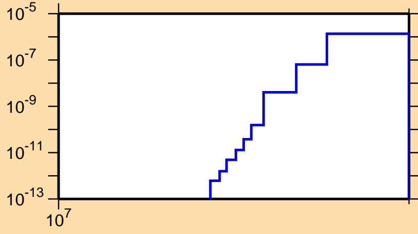
\sigma vs. E for ^{249}\text{Am}(n,\text{nd})
