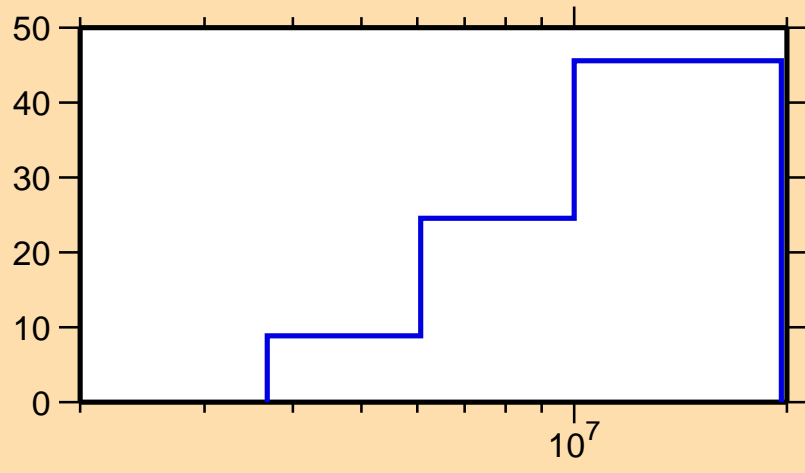
\Delta\sigma/\sigma vs. E for ^{249}\text{Am}(n,el.)
