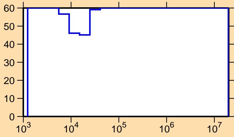
\Delta\sigma/\sigma vs. E for ^{249}\text{Am}(n,\gamma)
