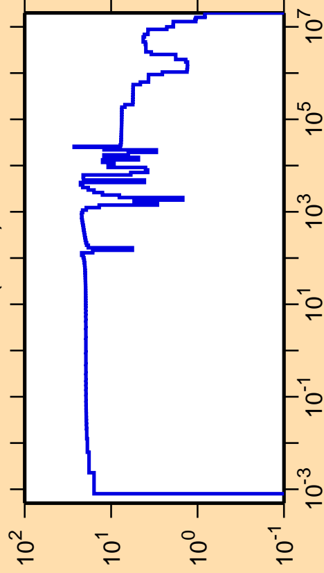
\Delta\sigma/\sigma vs. E for ^{35}\text{Ar}(n,\text{el.})
