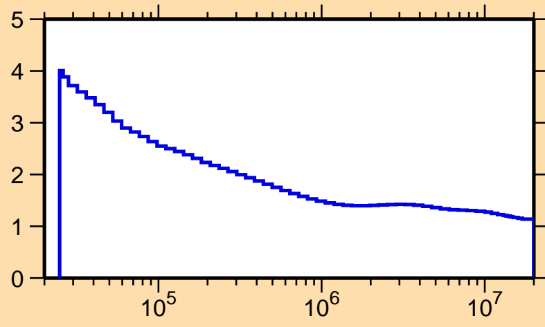
\sigma vs. E for ^{35}\text{Ar}(n,\text{nonel.})
