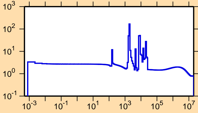
\sigma vs. E for ^{35}\text{Ar}(n,\text{el.})
