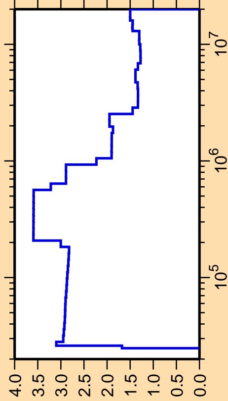
\Delta\sigma/\sigma vs. E for ^{35}\text{Ar}(n,\text{nonel.})
