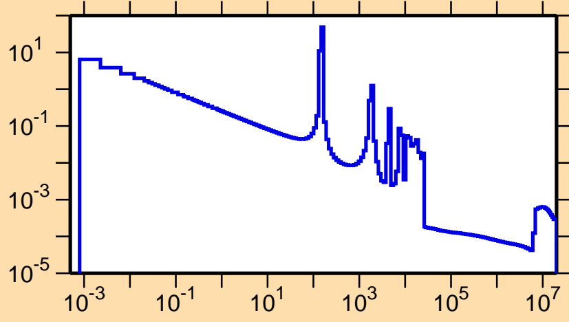
\sigma vs. E for ^{35}\text{Ar}(n,\gamma)
