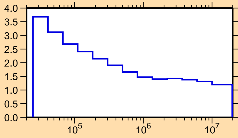
\sigma vs. E for ^{35}\text{Ar}(n,\text{nonel.})
