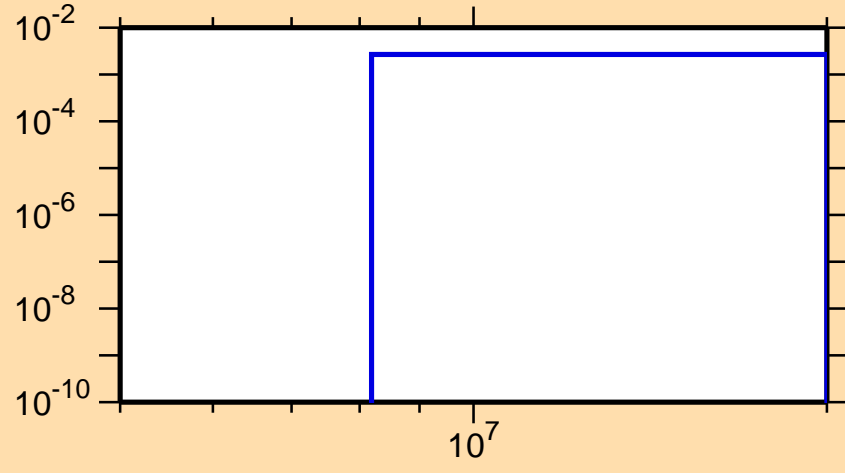
\sigma vs. E for ^{35}\text{Ar}(n,n\alpha)
