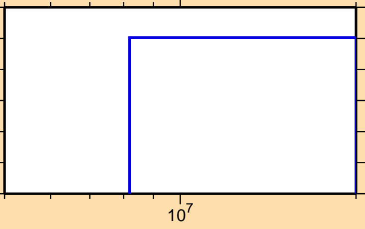
\sigma vs. E for ^{35}\text{Ar}(n,nd)
