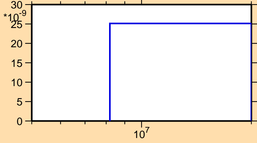
\sigma vs. E for ^{35}\text{Ar}(n,nd)
