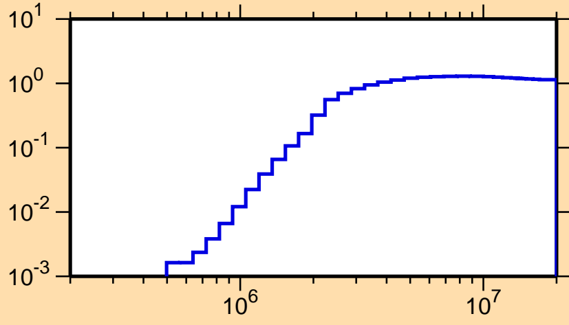
\sigma vs. E for ^{36}\text{Ar}(n,\text{nonel.})
